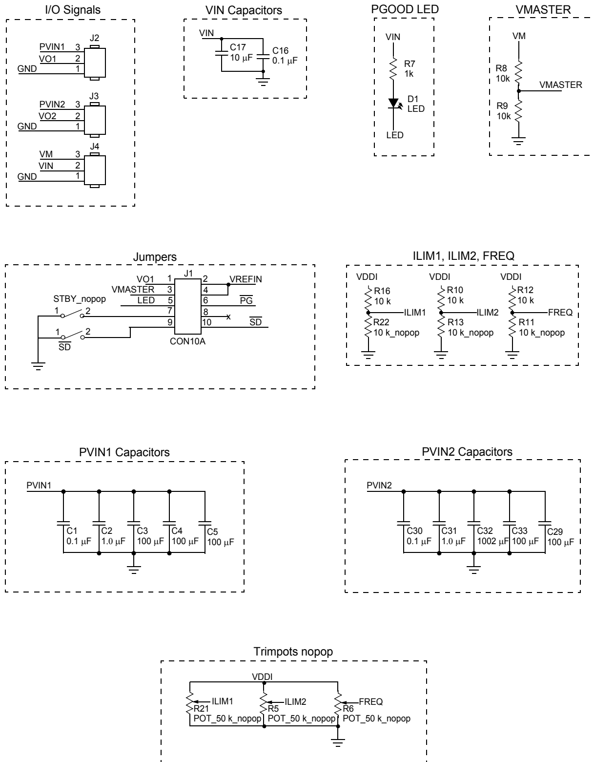
Figure 7. 34717 Typical Application
