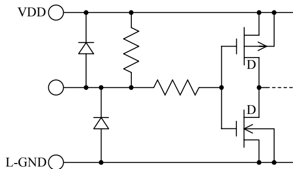
(b)LATCH,XEN
