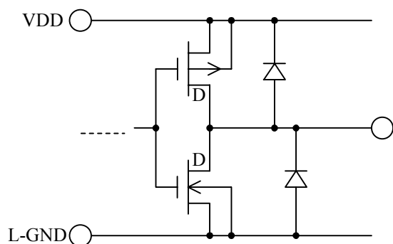
(c)S-OUT
