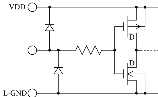
(a)CLK,S-IN
