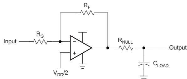
Figure 34. Driving a Capacitive Load
