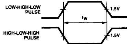
FIGURE 7. PULSE WIDTH
