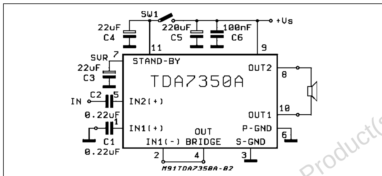
Figure 6. BRIDGE Test and Application Circuit
