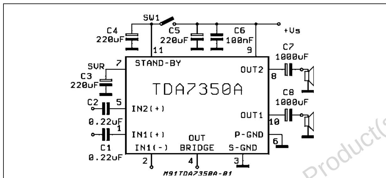
Figure 4. STEREO Test and Application Circuit
