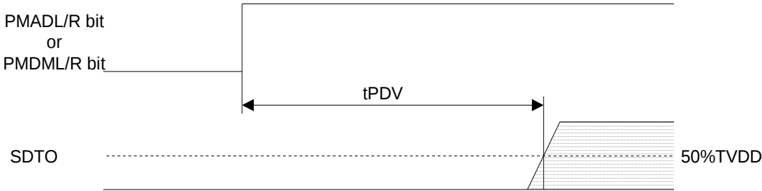
Figure 18. Power Down & Reset Timing 2
