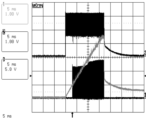
FIGURE 14. TYPICAL WAVEFORMS
