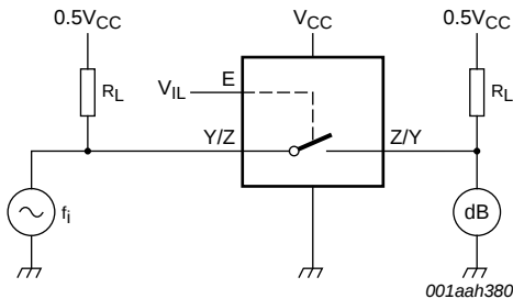
Fig 19. Test circuit for measuring isolation (OFF-state)
