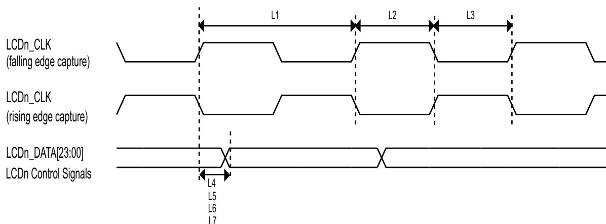
Figure 54. LCD Timing
