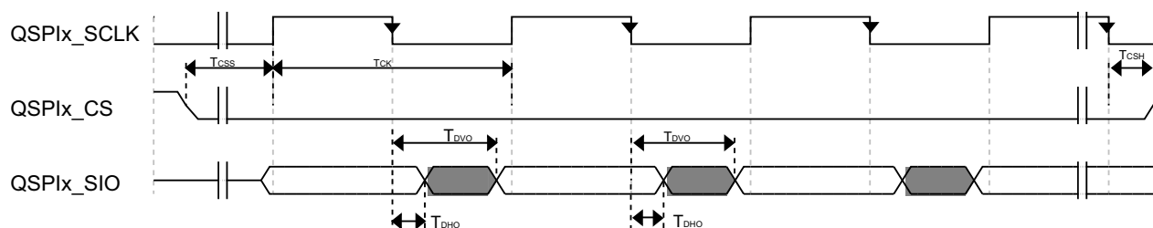
Figure 57. QuadSPI Output/Write Timing (SDR mode)
