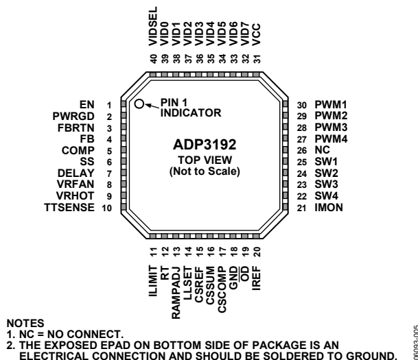
Figure 5. Pin Configuration
