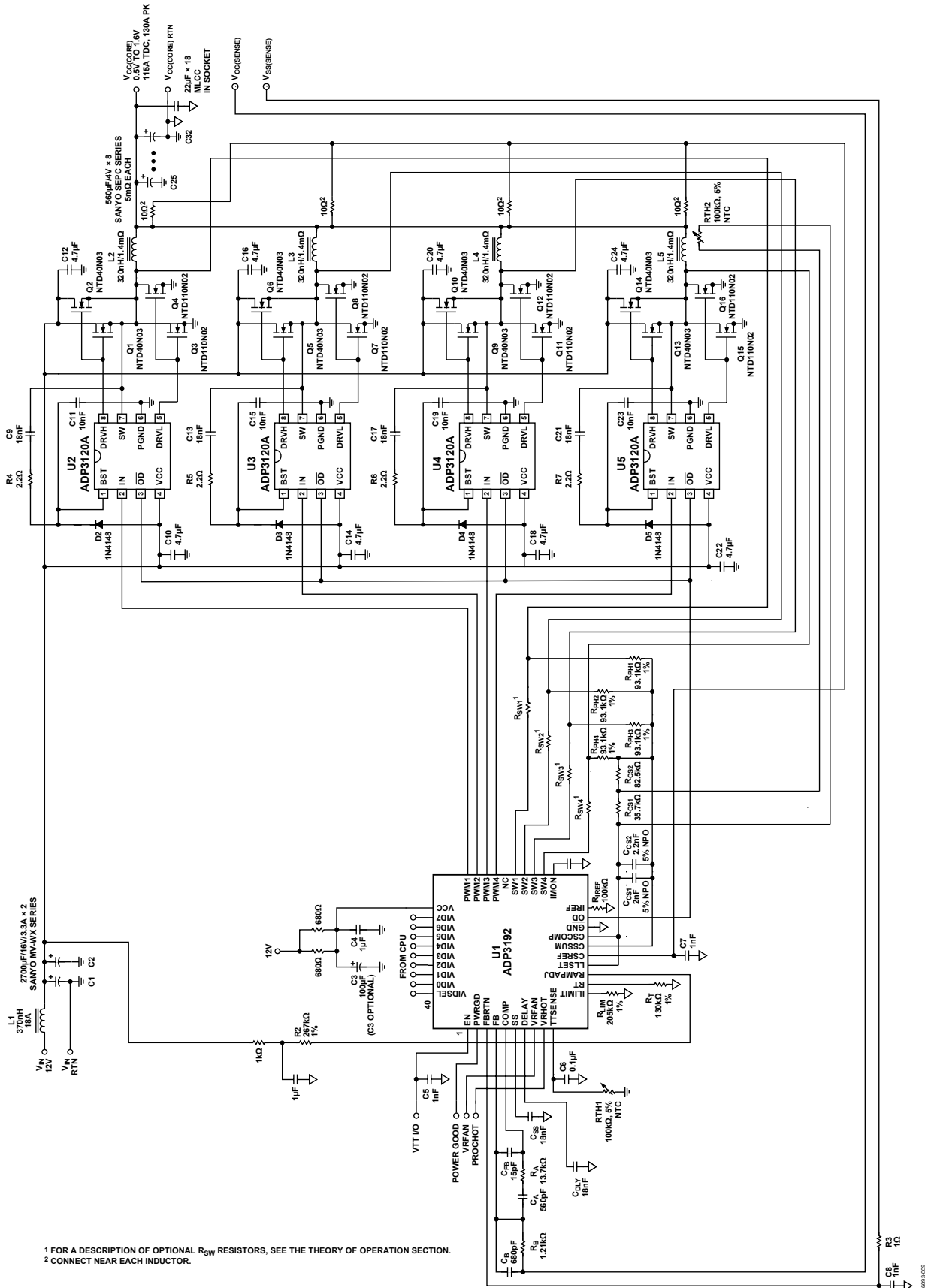
Figure 10. Typical 4-Phase Application Circuit
