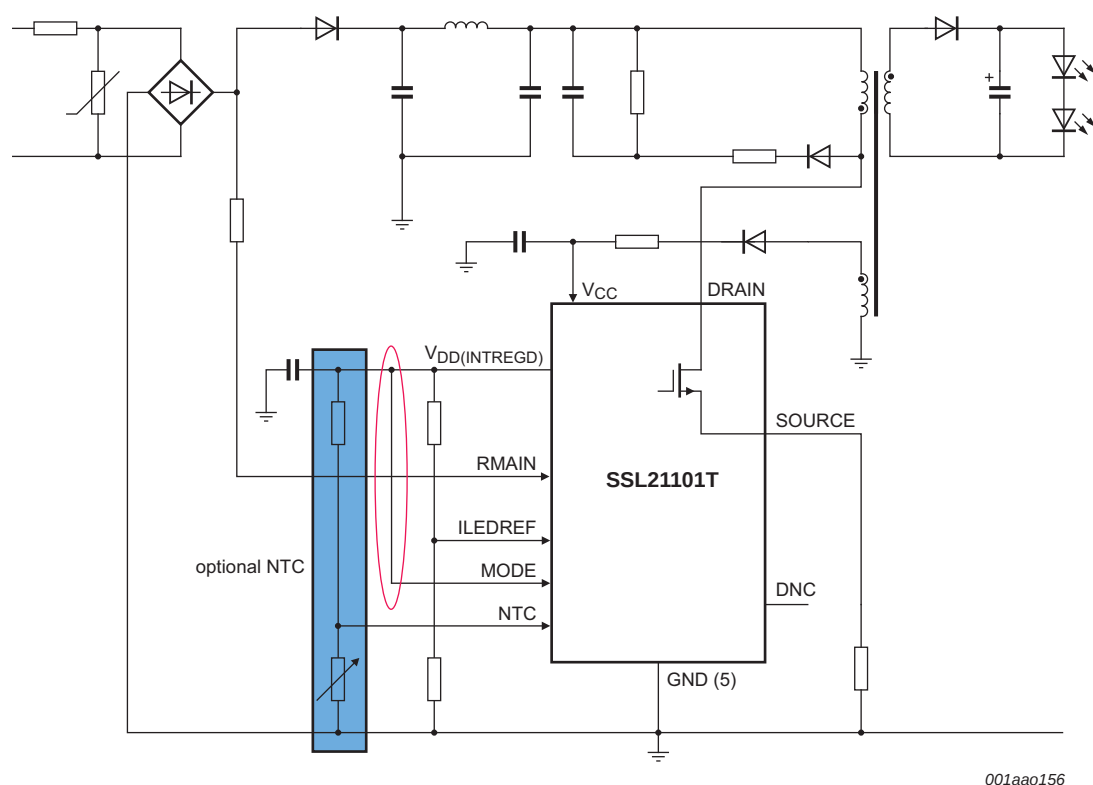
Fig 6. 100 kHz low THD application diagram
