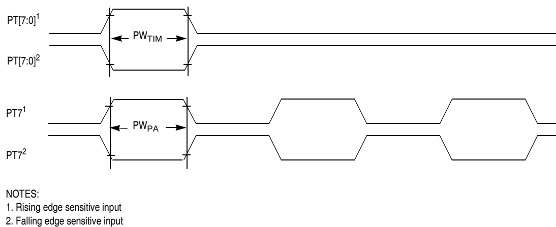
Figure 20-1. Timer Inputs
