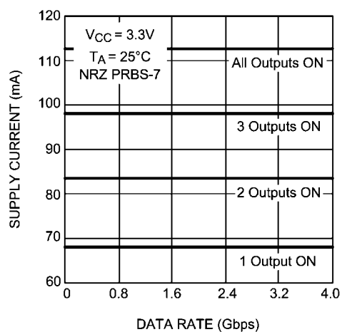
Supply Current as a Function of a Number of Outputs Used
