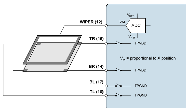
Figure 10 X Co-ordinate Measurement on 5-wire Touchpanel
