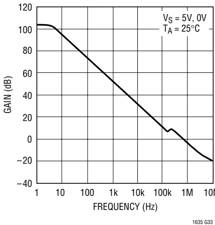
Reference Amplifier Gain
