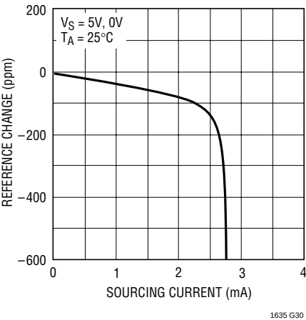
Load Regulation
