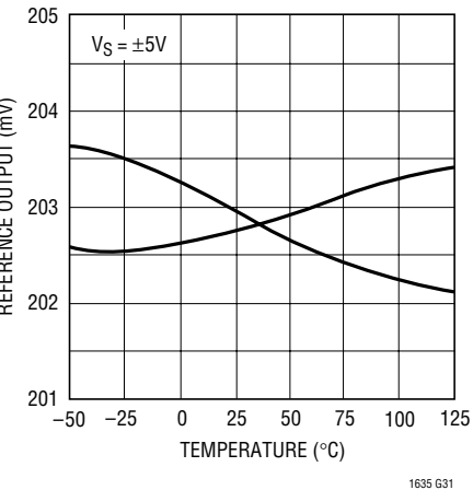
Reference Output vs Temperature of Two Typical Units
