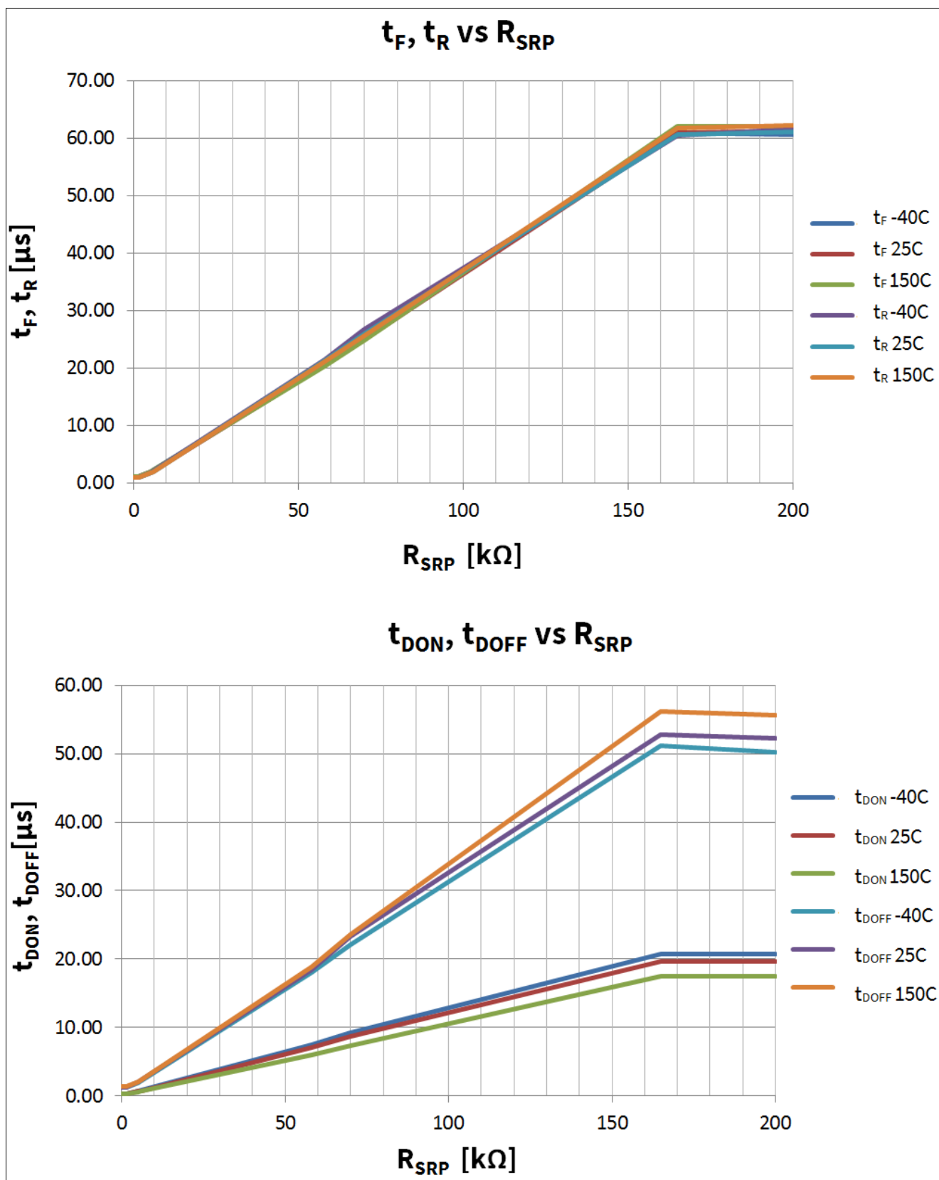
Figure 32 t_F, t_R, t_{DON}, t_{DOFF} vs. R_{SRP} ; V_{IN} = V_{ENABLE} = V_{DD} = 5V ; V_{BAT} = 13.5V ; R_L = 2.2\Omega ; T_J = -40, 25, 150^\circ C
