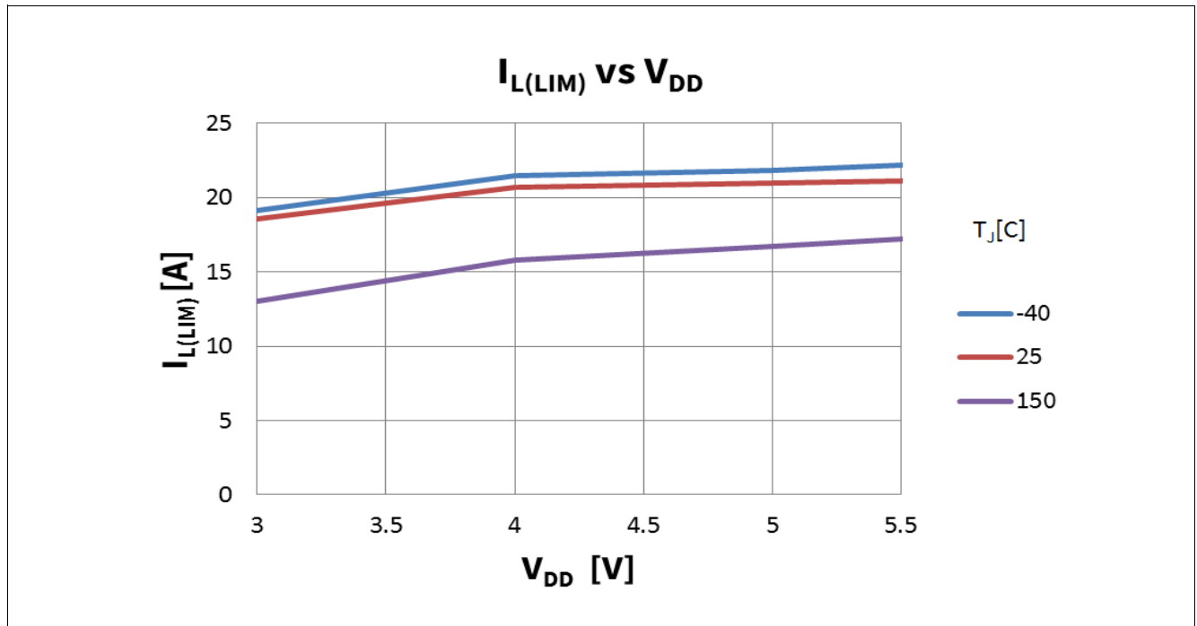
Figure 42 I_{L(LIM)} vs. V_{DD} = 3\text{V}...5.5\text{V} @ T_J = -40, 25, 150^\circ\text{C} ; V_{ENABLE} = V_{IN} = 5\text{V} ; V_{BAT} = 13.5\text{V}
