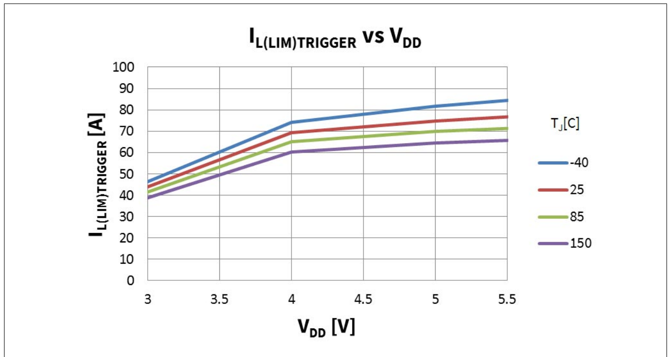
Figure 41 I_{L(LIM)TRIGGER} peak vs. V_{DD}=3...5.5\text{V} @ T_J = -40, 25, 85, 150^\circ\text{C} ; V_{IN} = \text{PWM } 5\text{V} in SOA; V_{ENABLE} = 5\text{V} ; V_{BAT} = 13.5\text{V} ; R_L = 2.2\Omega
