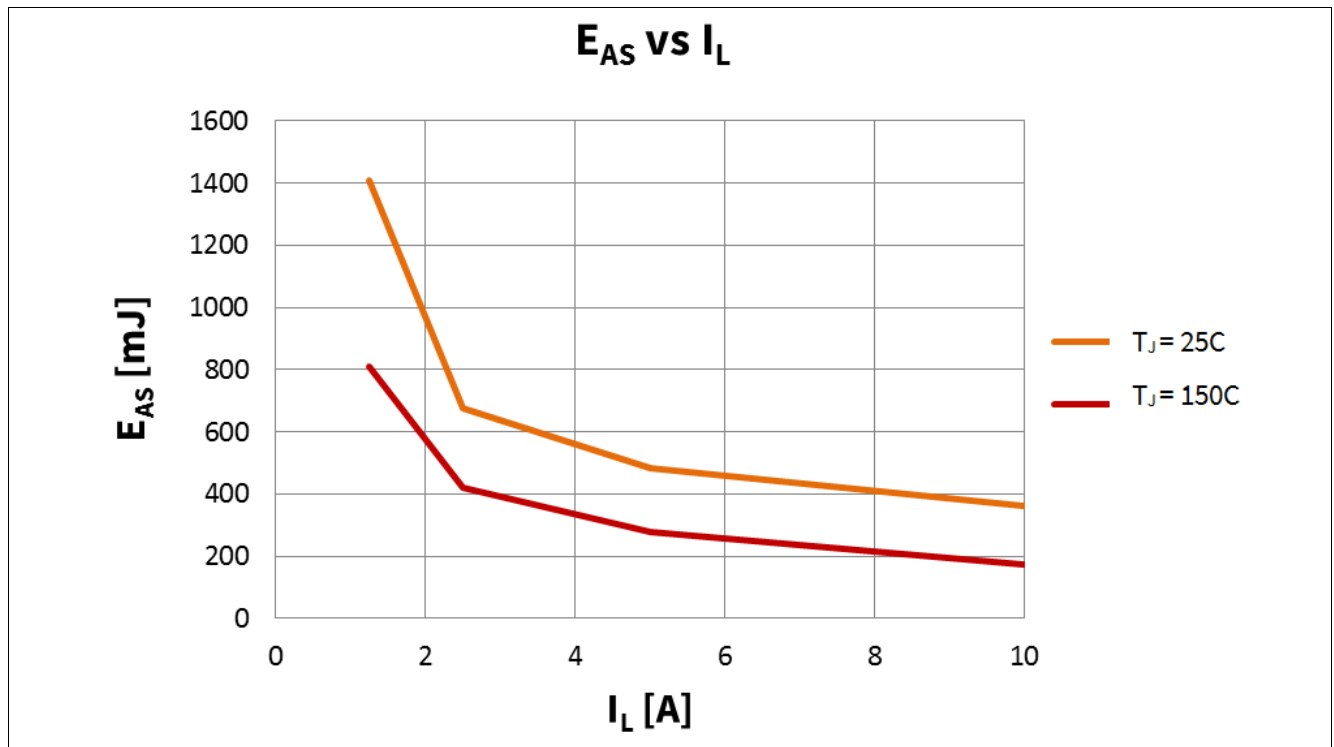
Figure 29 E_{AS} vs. I_L @ T_{J(0)}=25^\circ\text{C}, 150^\circ\text{C}, V_{BAT}=13.5\text{V}; V_{IN} = V_{ENABLE} = V_{DD} = \text{open}; I_L = I_{L(NOM)}/4, I_{L(NOM)}/2, I_{L(NOM)}, 2 \cdot I_{L(NOM)}
