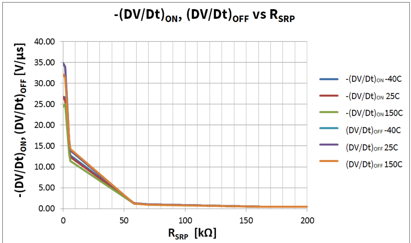
Figure 33 -(\Delta\text{V}/\Delta\text{t})_{\text{ON}}, (\Delta\text{V}/\Delta\text{t})_{\text{OFF}} vs. R_{\text{SRP}} ; V_{\text{IN}} = V_{\text{ENABLE}} = V_{\text{DD}} = 5\text{V} ; V_{\text{BAT}} = 13.5\text{V} ; R_{\text{L}} = 2.2\Omega ; T_{\text{J}} = -40, 25, 150^\circ\text{C}
