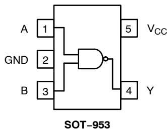
Figure 2. Pinout (Top View)
