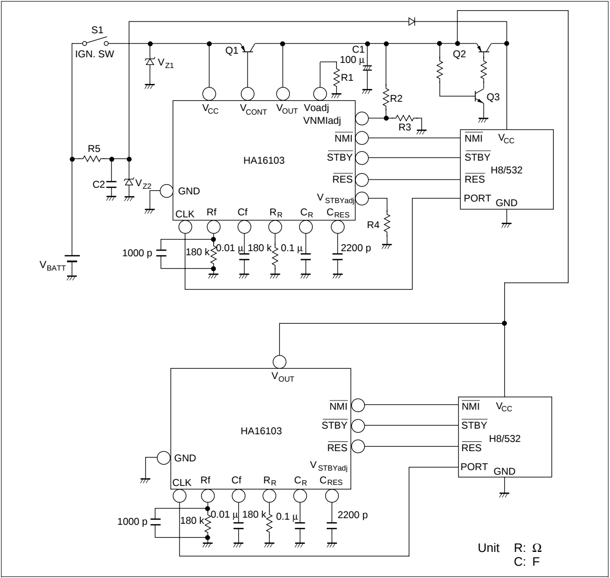
Sample Connection Circuit between HA16103 and H8/532 (2)
