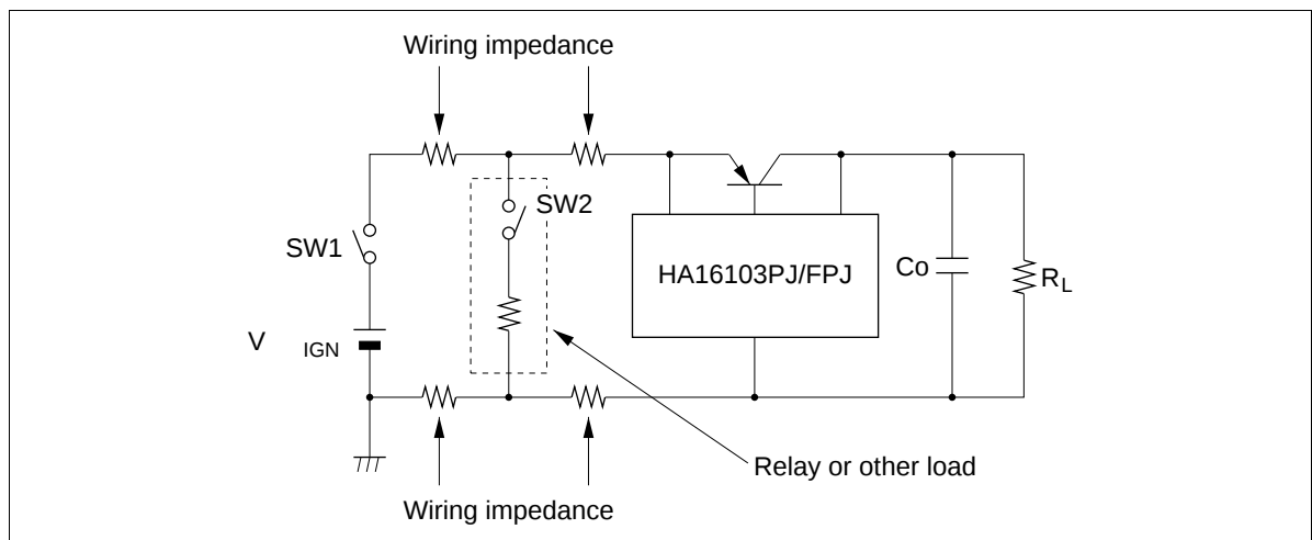
Figure 6 Typical Circuit
