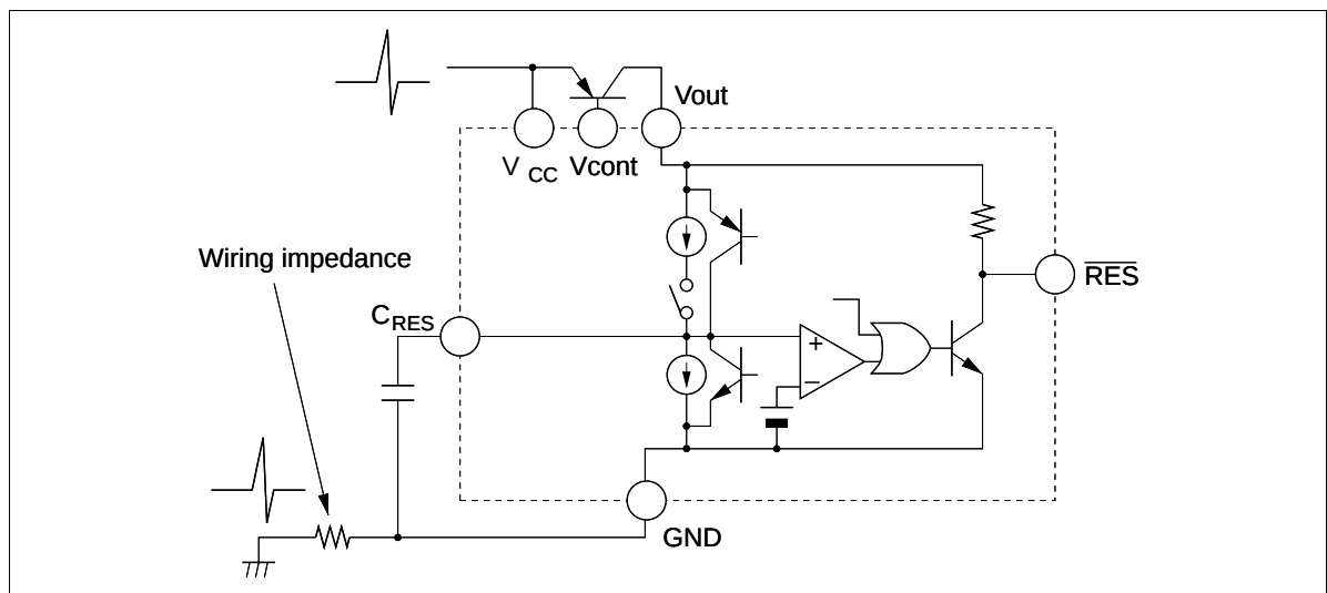
Figure 7 \overline{\text{RES}} Comparator
