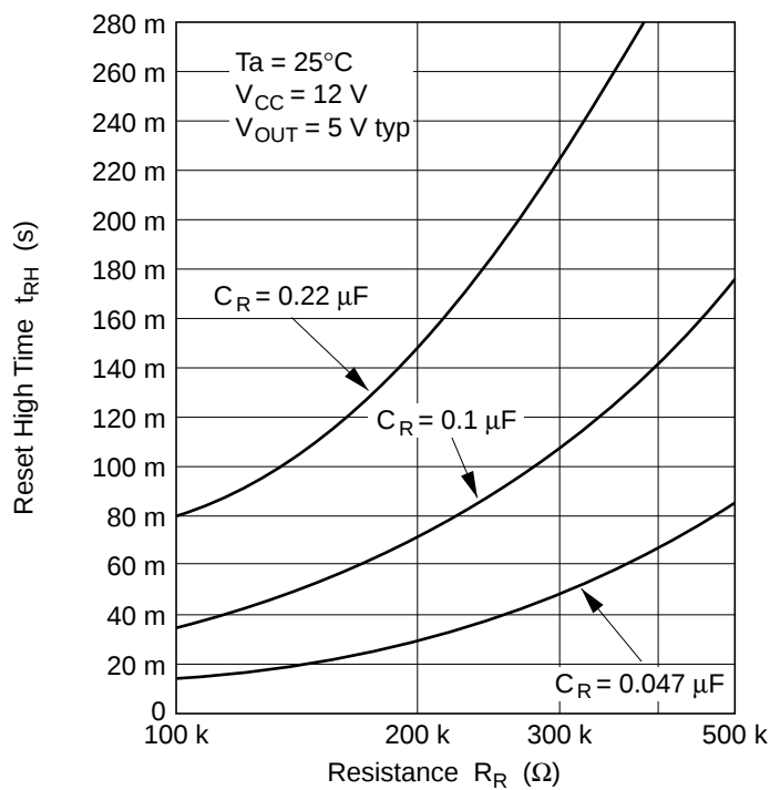
• Power-on and auto-reset section Reset High Time vs. Resistance R_R
