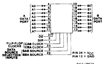
FUNCTIONAL DIAGRAM
