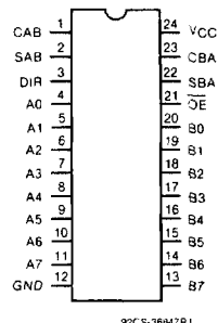
TERMINAL ASSIGNMENT
