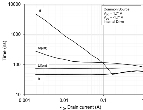
Figure 125: Typical Switching Time (Internal Gate Drive) at V_{DS} = 1.71 V
