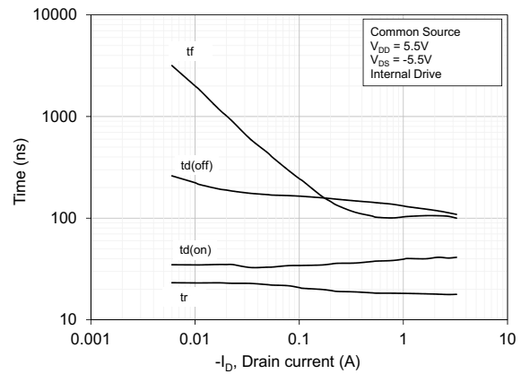
Figure 126: Typical Switching Time (Internal Gate Drive) at V_{DS} = 5.5 V
