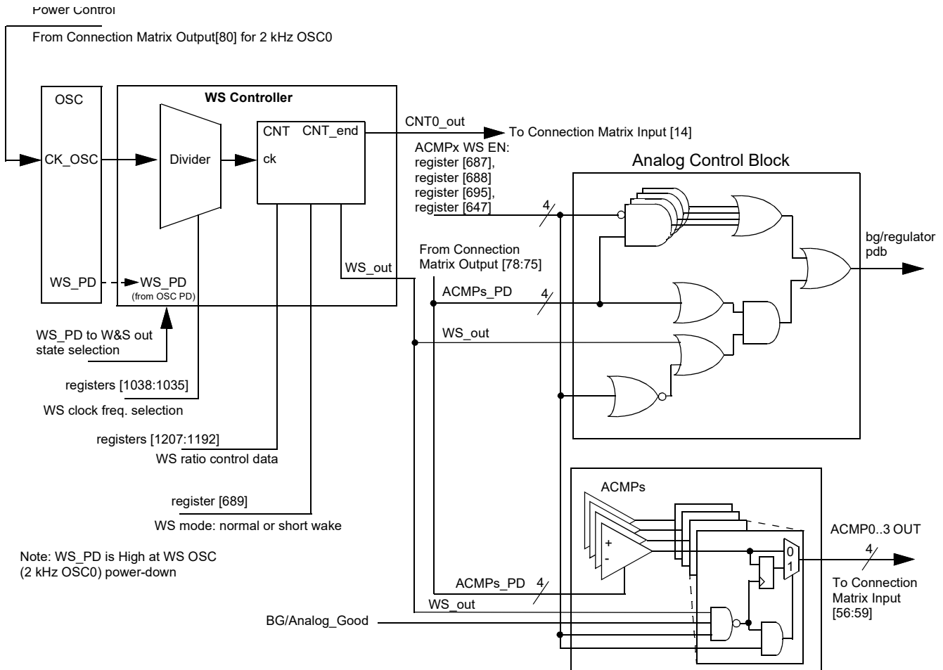
Figure 57: Wake/Sleep Controller
