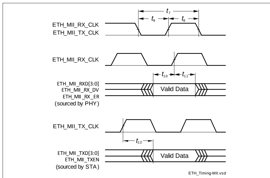
Figure 53 ETH MII Signal Timing
