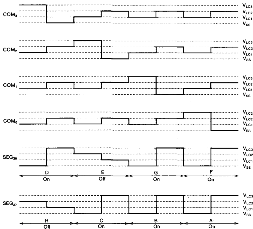
Fig. 38 Display pattern example and drive waveform example
