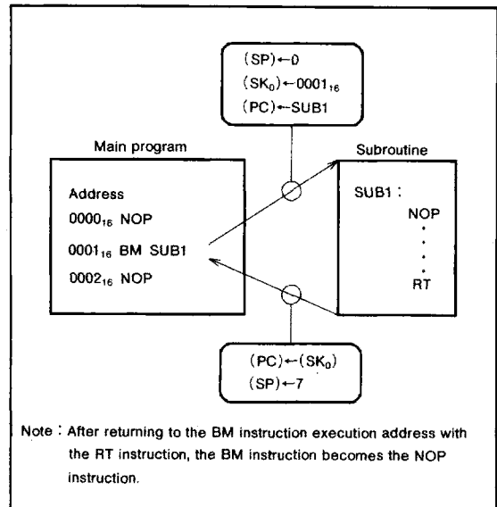
Fig. 6 Operation at subroutine call
