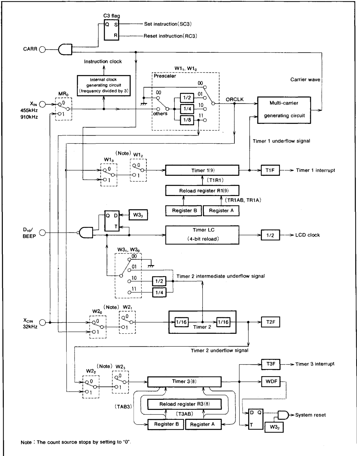
Fig. 19 Timers structure
