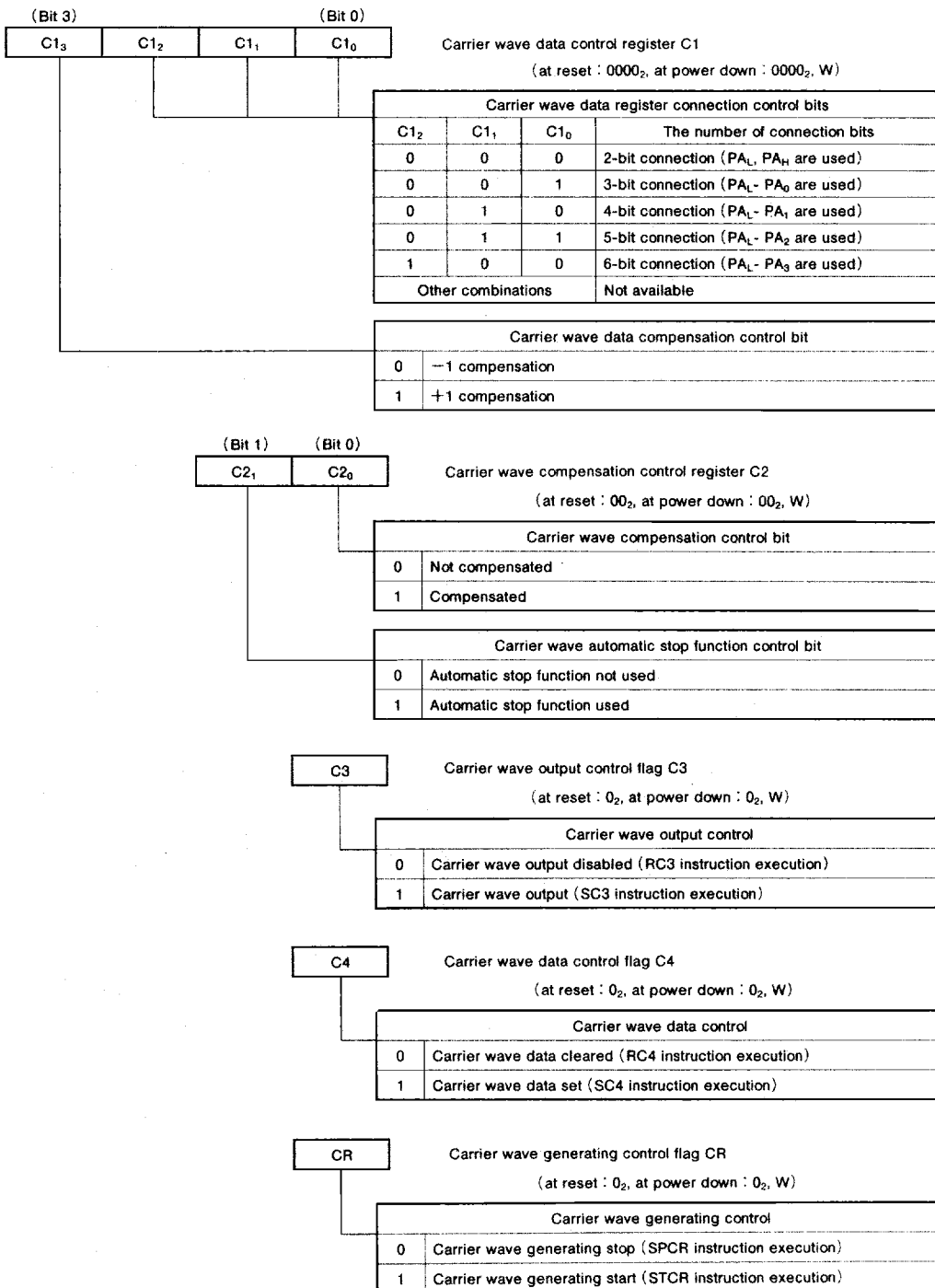
Fig. 25 Multi-carrier generating circuit control register and control flag
