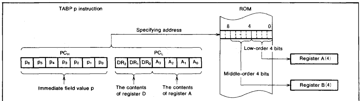
Fig. 4 TABP p instruction execution example
