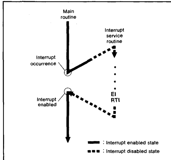
Fig. 16 Program example of interrupt processing
