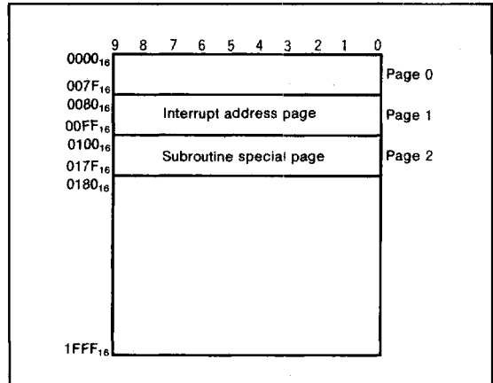
Fig. 7 ROM map of M34550M8A-XXXXFP
