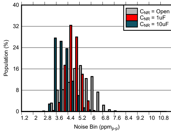
Figure 7-9. 0.1 Hz to 10 Hz Noise Distribution ( V_{REF} = 2.5\text{ V} , C_L = 1\text{ }\mu\text{F} , I_L = 0\text{ mA} )
