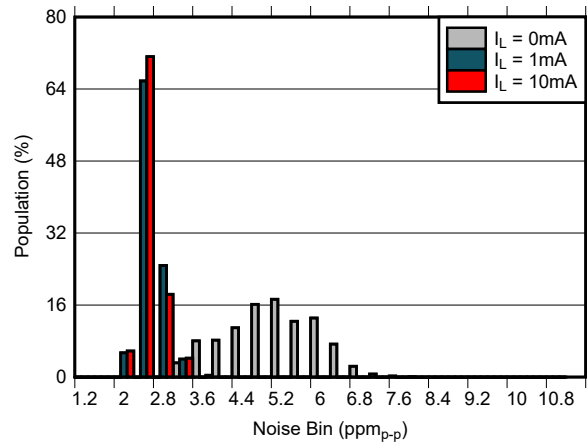
Figure 7-10. 0.1 Hz to 10 Hz Noise Distribution ( V_{REF} = 2.5\text{ V} , C_L = 1\text{ }\mu\text{F} , C_{NR} = \text{Open} )
