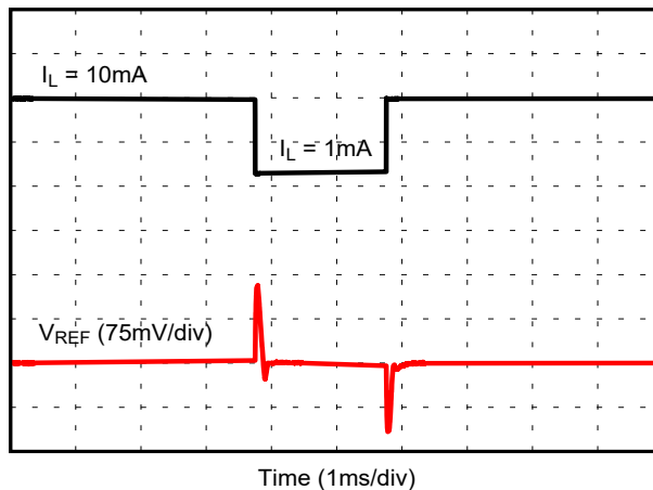
Figure 9-4. Load Transient Response 1 mA to 10 mA, C_L = 1 \mu F
