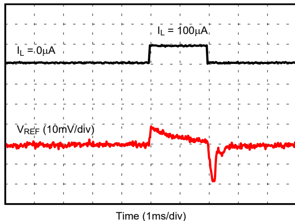
Figure 9-3. Load Transient Response 0 \mu A to 100 \mu A, C_L = 1 \mu F
