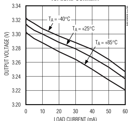
BKSU OUTPUT VOLTAGE vs. LOAD CURRENT
