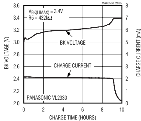
CHARGE PROFILE FOR LiFeO5
