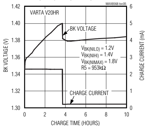
CHARGE PROFILE FOR NiMH
