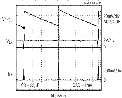
LIGHT-LOAD SWITCHING WAVEFORMS
