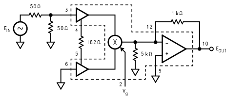
FIGURE 6. Typical Circuit
