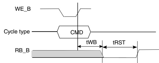
Figure 52. t_{WB} , t_{RST} Timings
