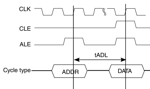
Figure 61. tADL Timings
