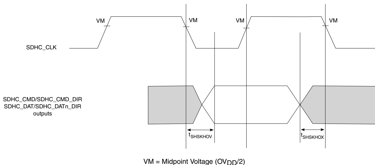
Figure 73. eSDHC high-speed mode output AC timing diagram
