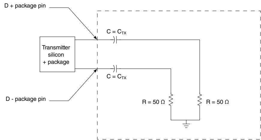
Figure 96. Test and measurement load
