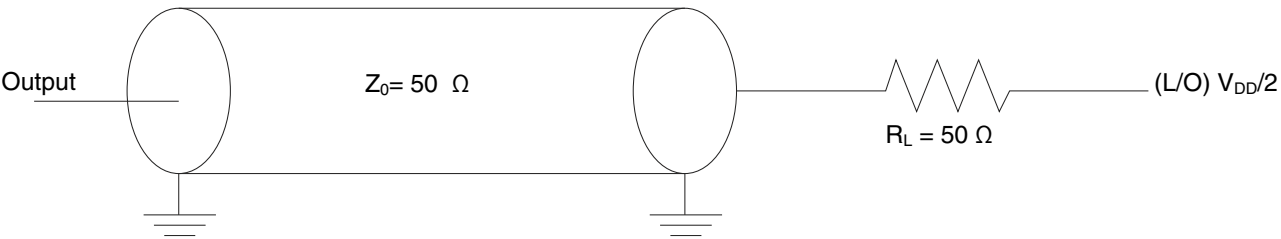
Figure 67. Flextimer AC test load
