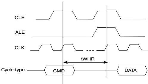
Figure 65. t_{WHR} Timings
