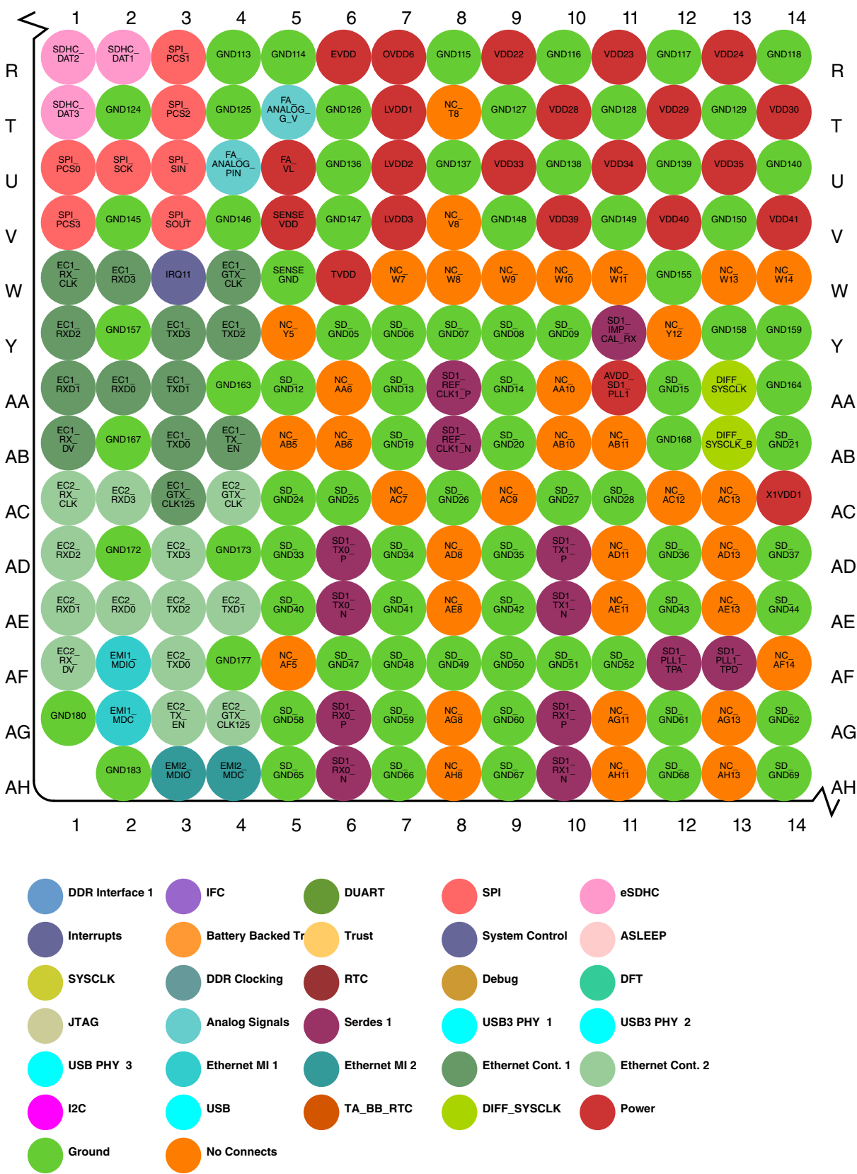
Figure 11. Detail C
