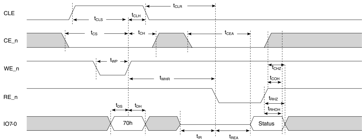
Figure 49. Read StatusTimings
