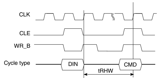
Figure 50. t_{RHW} Timings
