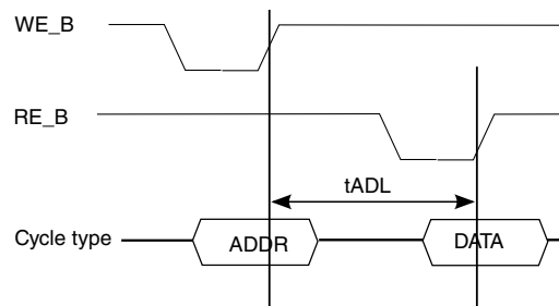
Figure 43. tADL Timing
