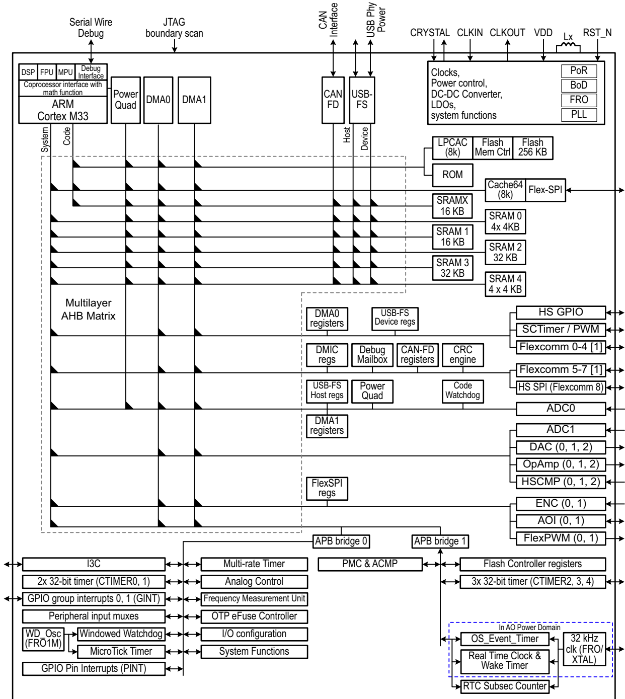
Fig 3. LPC553x Block diagram (Non-secure)
