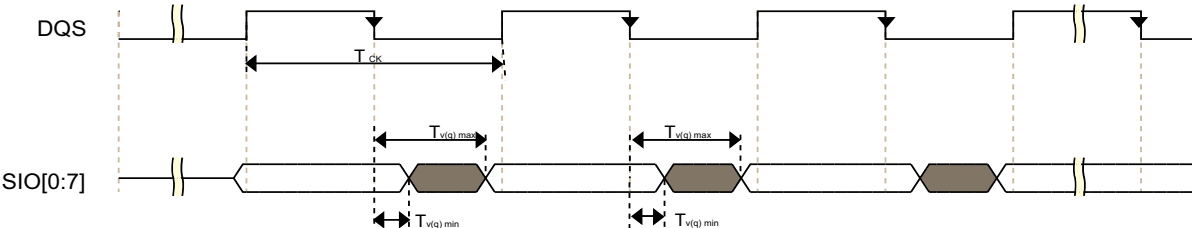
Fig 26. SDR mode (output timing, mode 3)
