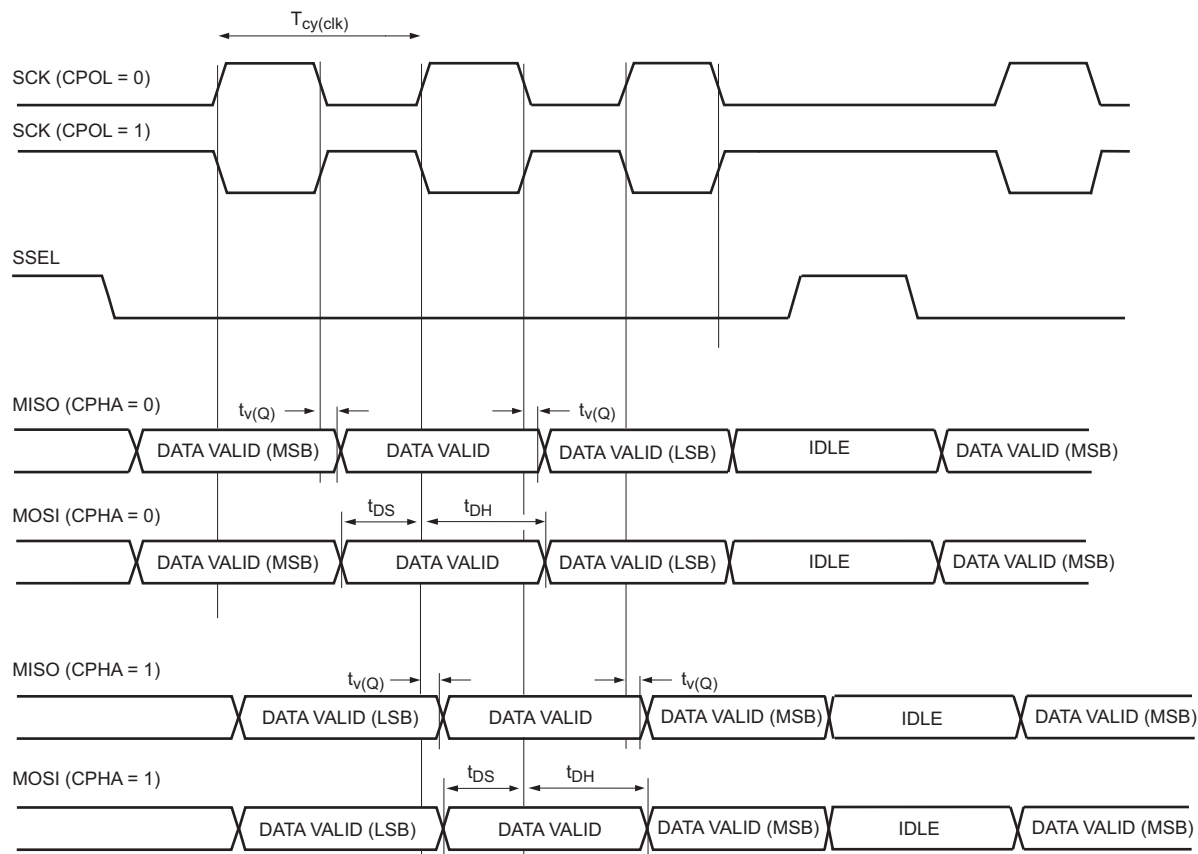
Fig 21. SPI slave timing
