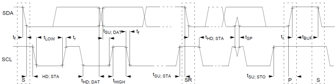
Fig 15. Timing definition for devices on the I 2 C bus
