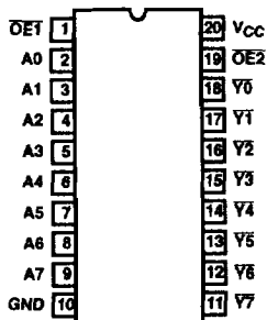
CD74FCT540 (PDIP, SOIC) TOP VIEW
