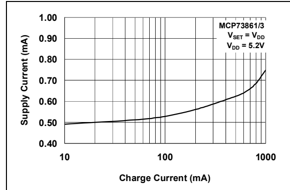
FIGURE 2-4: Supply Current ( I_{SS} ) vs. Charge Current ( I_{OUT} ).
