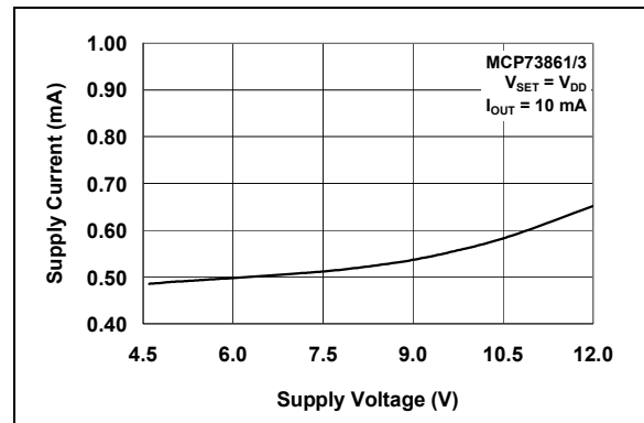
FIGURE 2-6: Supply Current ( I_{SS} ) vs. Supply Voltage ( V_{DD} ).
