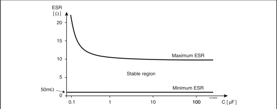
Figure 9. Maximum ESR for stability (valid for all the regulator outputs)
