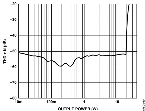
Figure 11. THD + N vs. Output Power, 15 V, 4 \Omega
