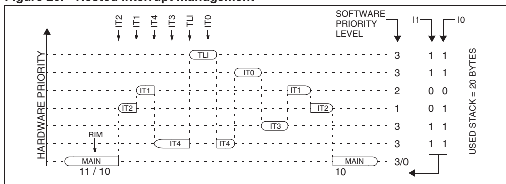
Figure 20. Nested interrupt management
