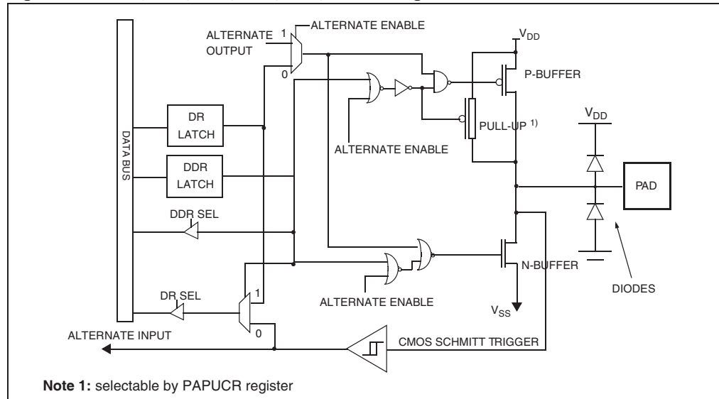
Figure 23. PA0, PA1, PA2, PA3, PA4, PA5 configuration
