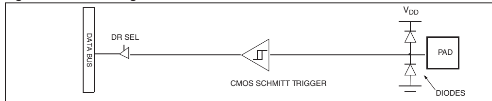
Figure 24. PA6 configuration
