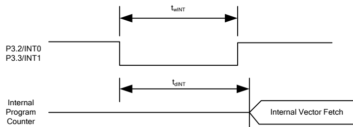
Figure 8 Interrupt timing
