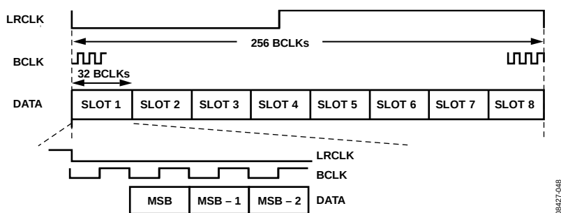
Figure 49. TDM Mode
