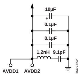
Figure 53. GSM Filter on the Analog Supply Pins
