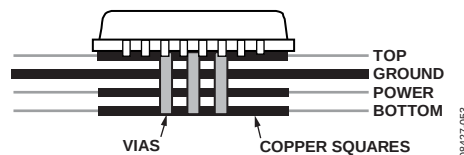
Figure 54. Exposed Pad Layout Example, Side View
