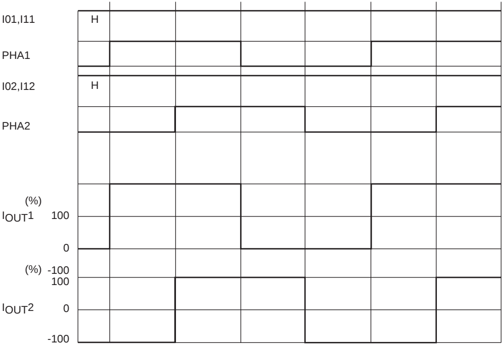
(6) Current waveforms in the various commutation modes 2-phase commutation (Channels 1 and 2, CW mode)
