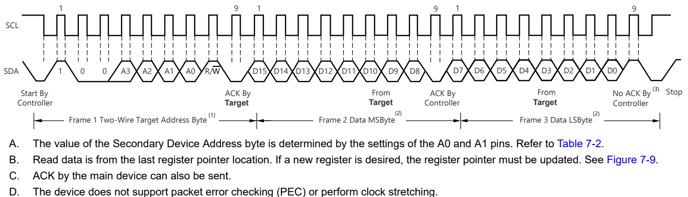
Figure 7-8. Timing Diagram for Read Word Format
