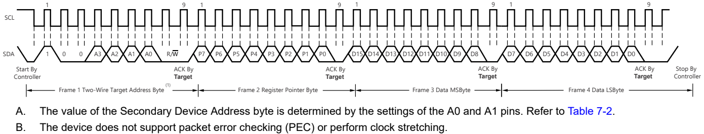
Figure 7-7. Timing Diagram for Write Word Format
