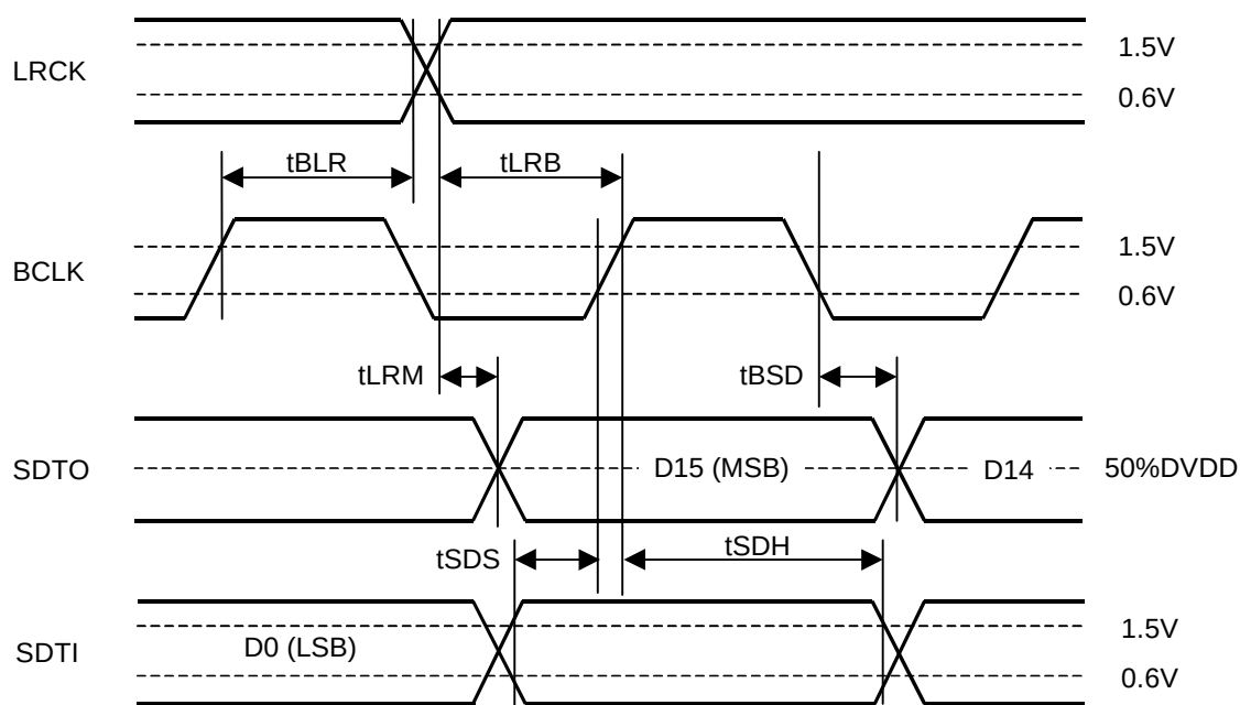
Figure 3. Clock Timing
