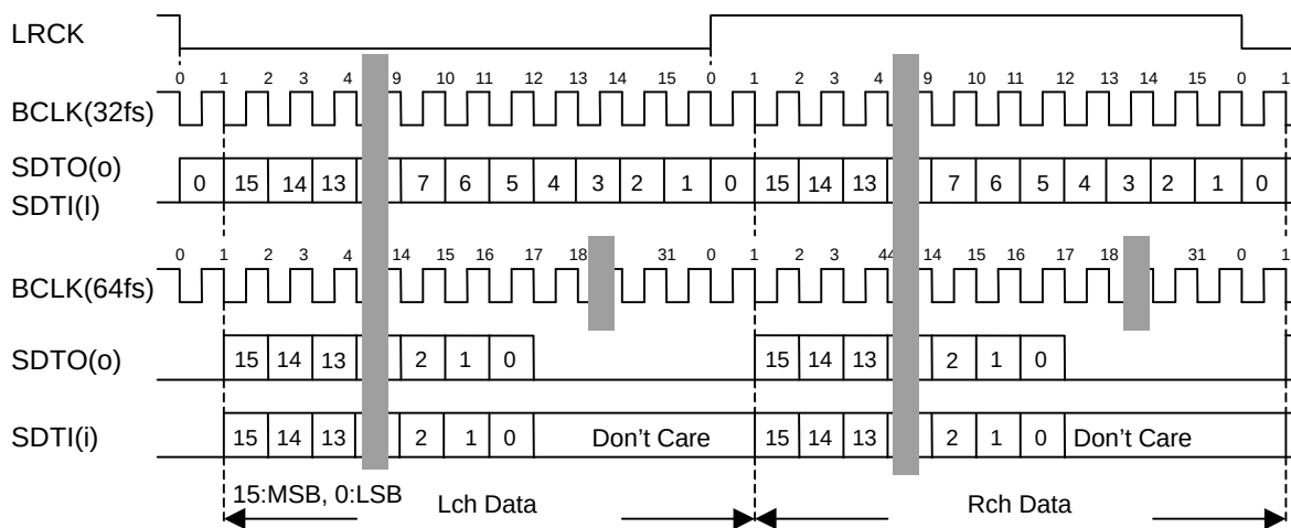
Figure 11. Audio Data Timing (No.3)
