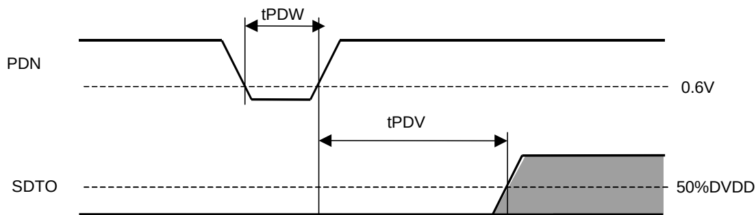
Figure 7. Reset Timing
