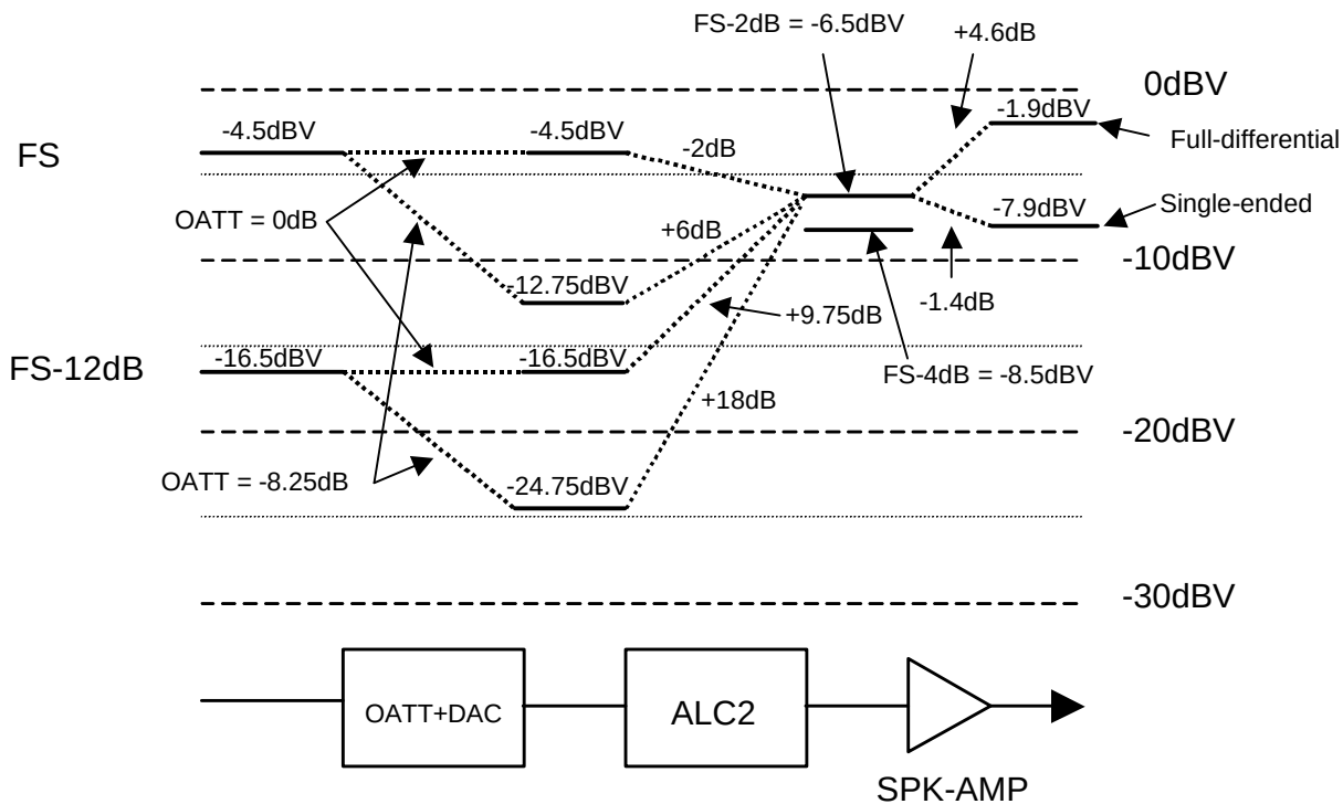
Figure 19. Speaker-Amp Output Level Diagram (AVDD=2.8V, OATT= -8.25dB &amp; 0dB)
