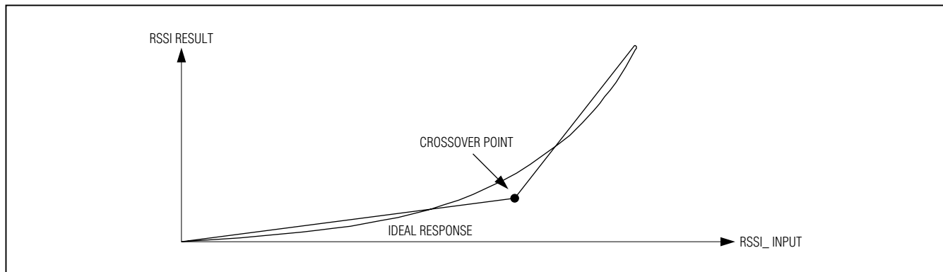
Figure 5. Crossover Enabled
