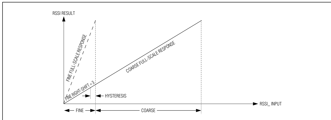
Figure 6. Crossover Disabled
