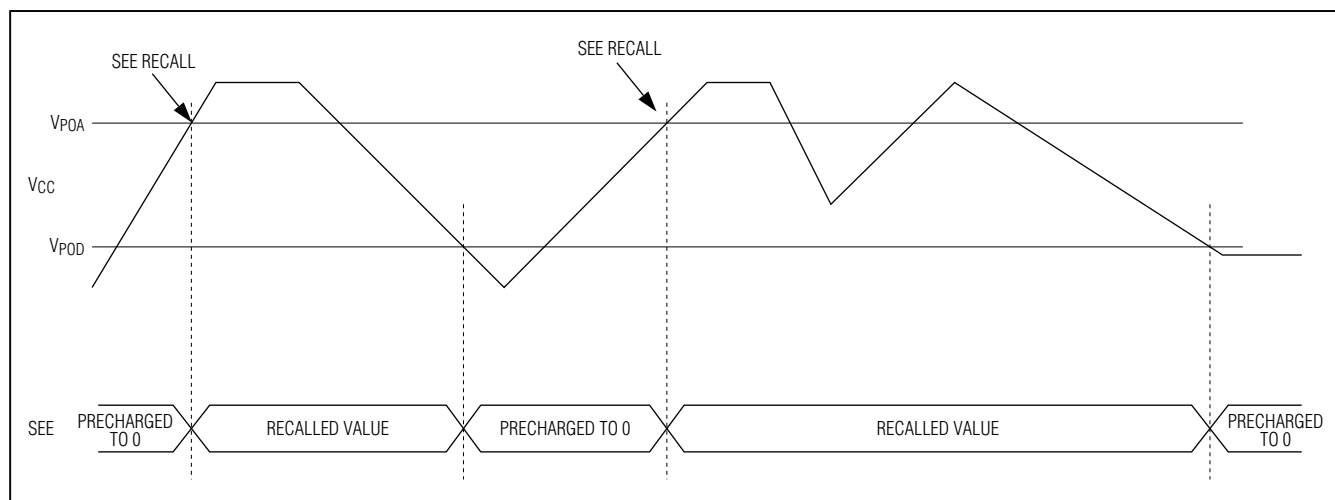
Figure 7. Low-Voltage Operation
