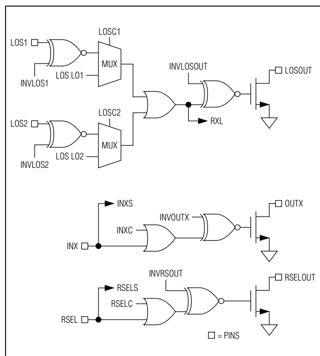
Figure 11. Logic Diagram
