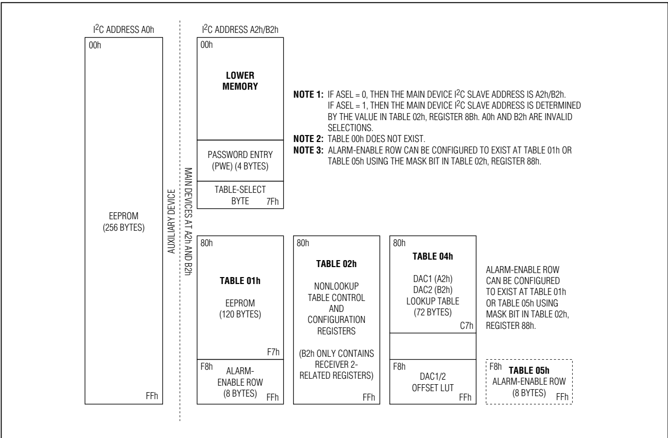
Figure 14. Memory Map
