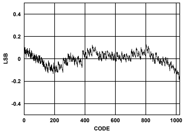
FIGURE 37. INTEGRAL NONLINEARITY
