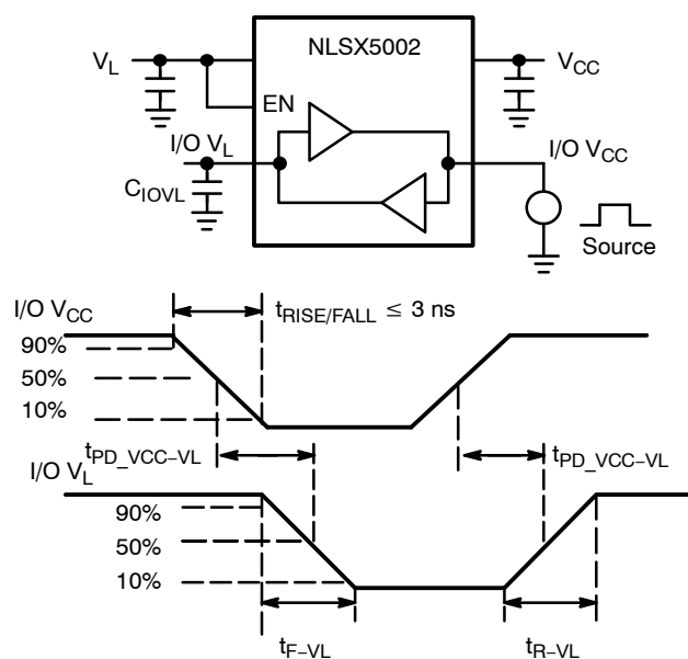
Figure 8. Driving I/O V_L Test Circuit and Timing
