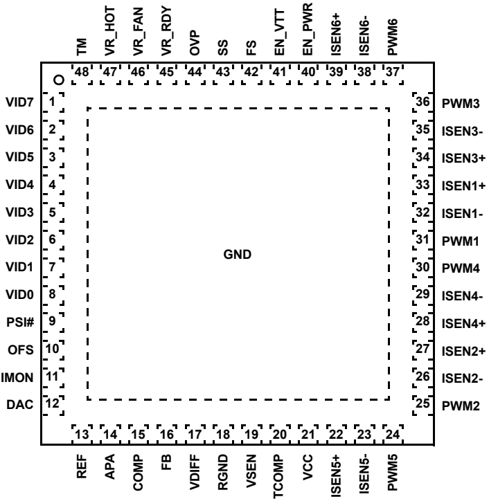
ISL6336, ISL6336A (48 LD QFN) TOP VIEW
