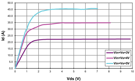
Figure 10. Output characteristics ( T_{case} = 25\text{ }^{\circ}\text{C} )
