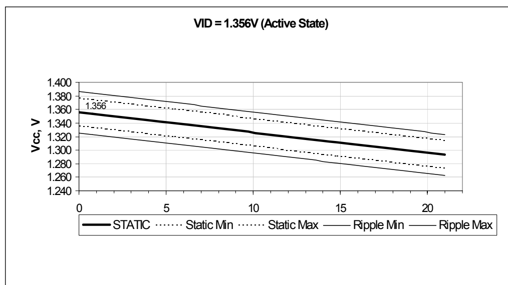
Figure 2. Illustration of Active State V_{\text{CC}} Static and Ripple Tolerances
