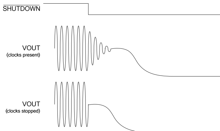
Figure 23 SHUTDOWN Operation
