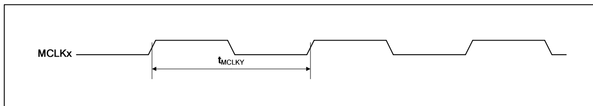
Figure 1 MCLK Timing
