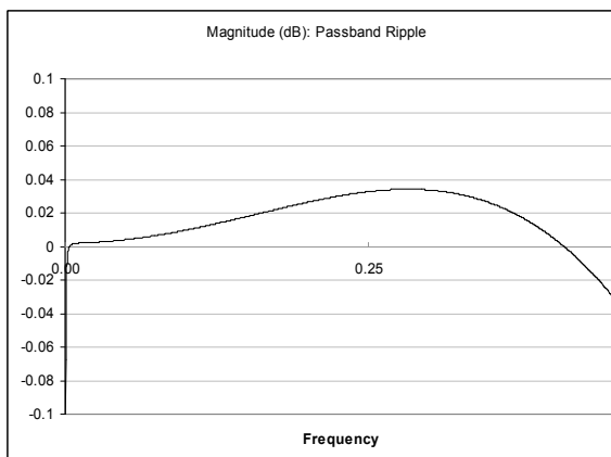
Figure 67 ADC Digital Filter Ripple
