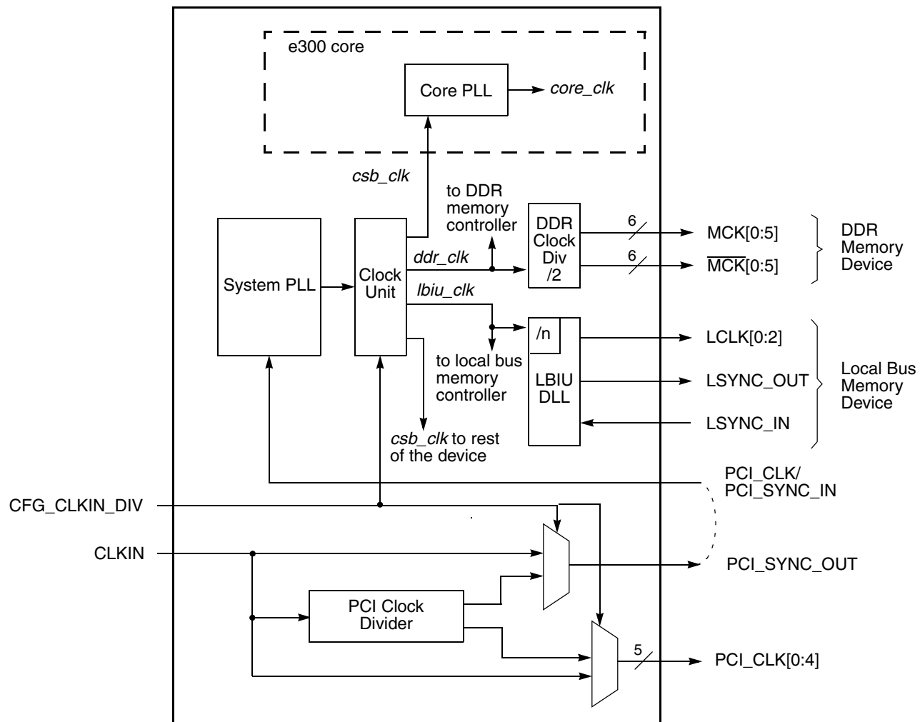
Figure 67. Clock Subsystem
