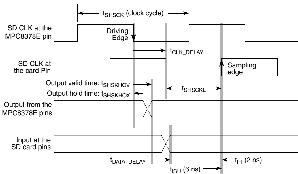
Figure 34. High Speed Output Path
