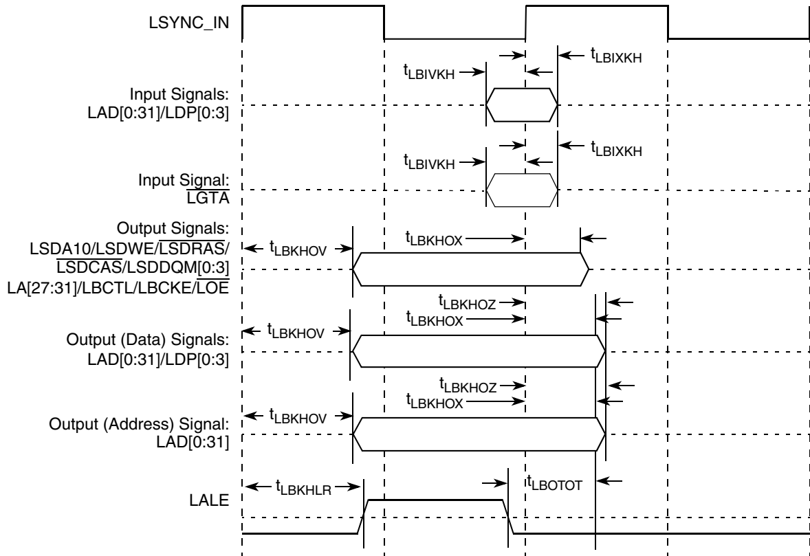
Figure 24. Local Bus Signals, Non-special Signals Only (PLL Enable Mode)
