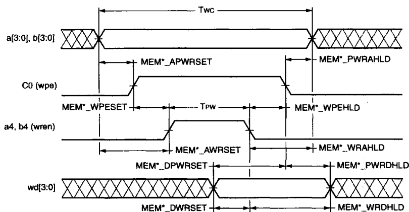
Figure 58. Write Operation
