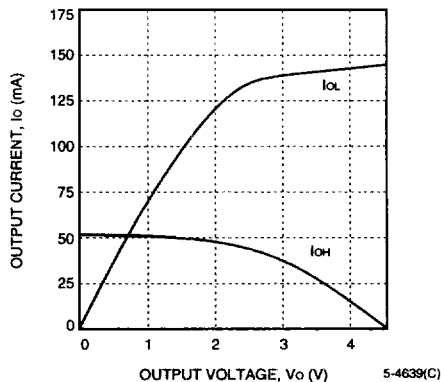
Figure 83. Fast ( T_J = 125^\circ\text{C} , V_{DD} = 4.5\text{ V} )
