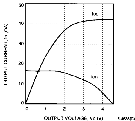
Figure 81. Sinklim ( T_J = 125^\circ\text{C} , V_{DD} = 4.5\text{ V} )
