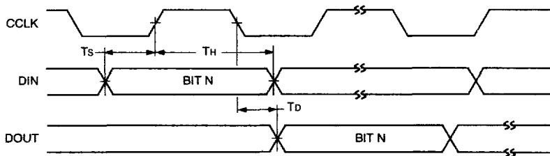
Figure 67. Master Serial Configuration Mode Timing Diagram
