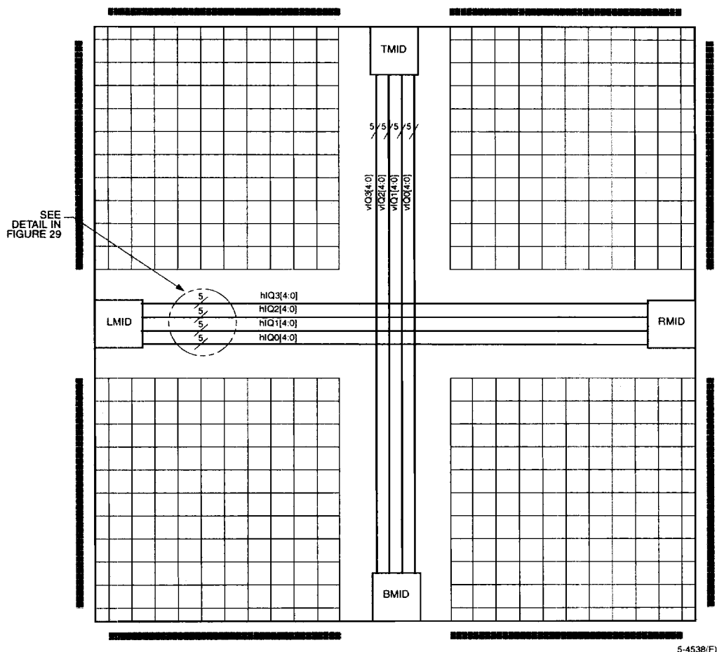
Figure 28. Interquad Routing
