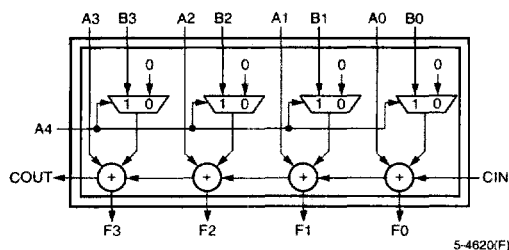
Figure 11. Multiplier Submode
