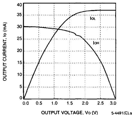
Figure 87. Sinklim ( T_J = 125^\circ\text{C} , V_{DD} = 3.0\text{ V} )
