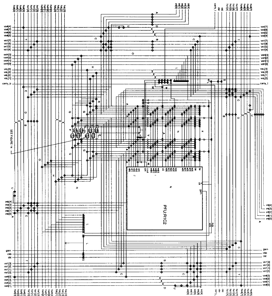
Figure 23. PLC Architecture
