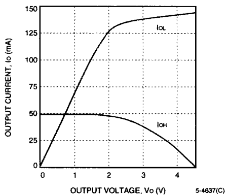
Figure 82. Slewlim ( T_J = 125^\circ\text{C} , V_{DD} = 4.5\text{ V} )
