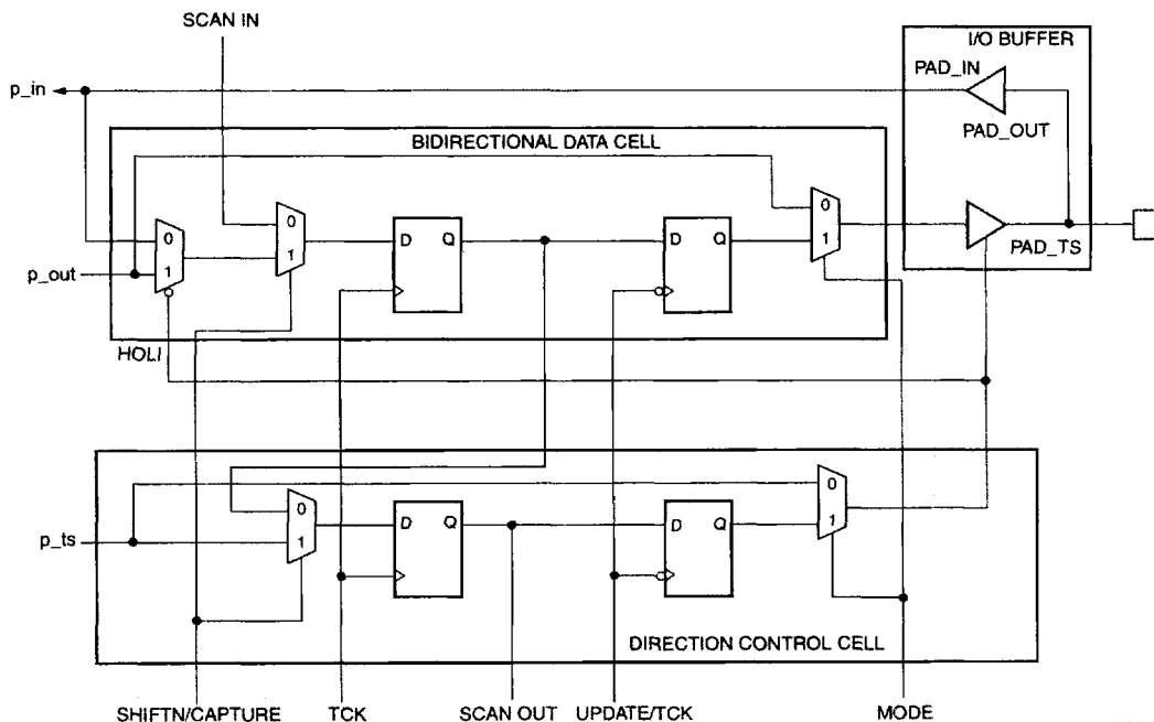
Figure 52. Boundary-Scan Cell
