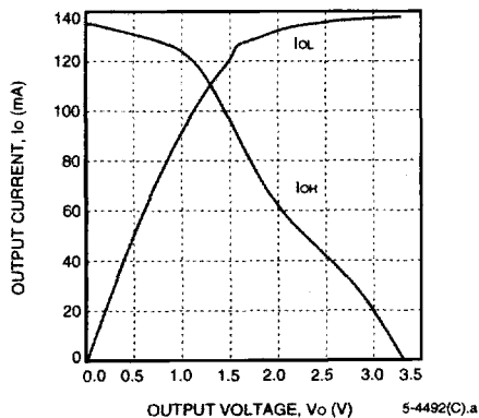
Figure 86. Fast ( T_J = 25^\circ\text{C} , V_{DD} = 3.3\text{ V} ) Lucent Technologies Inc.
