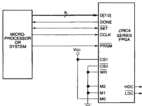
Figure 46. Slave Parallel Configuration Schematic
