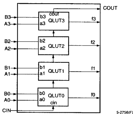
Figure 9. Ripple Mode
