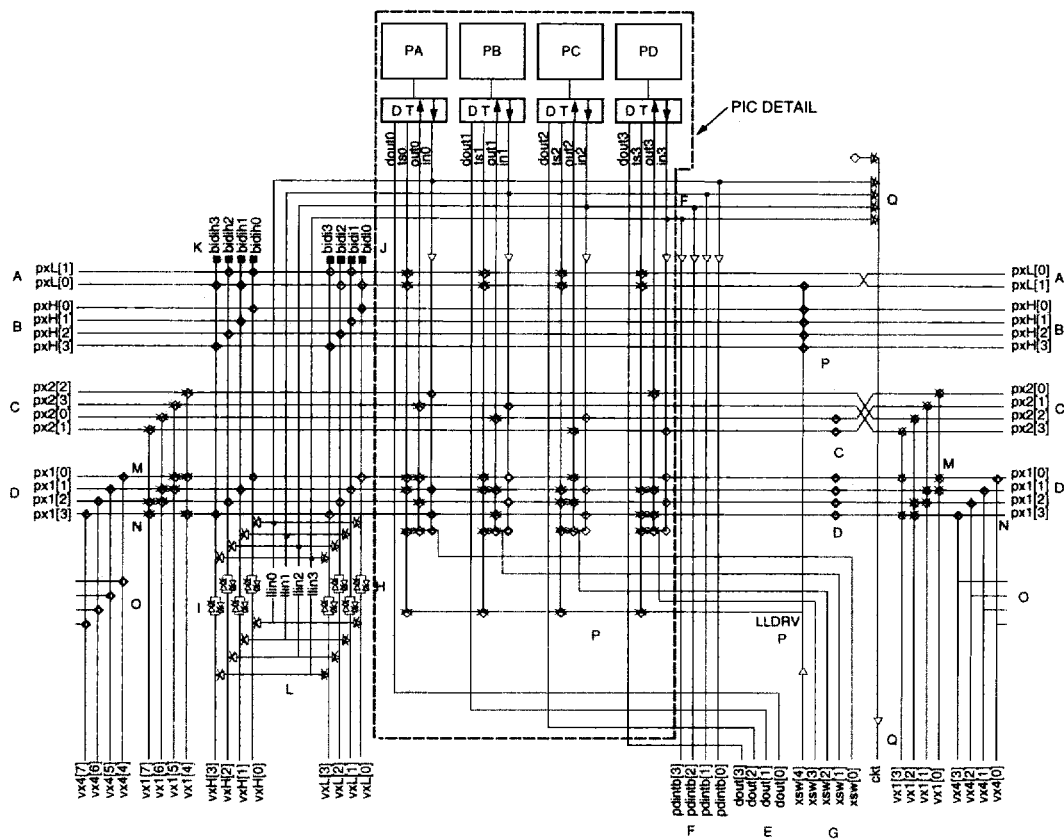
Figure 26. PIC Architecture
