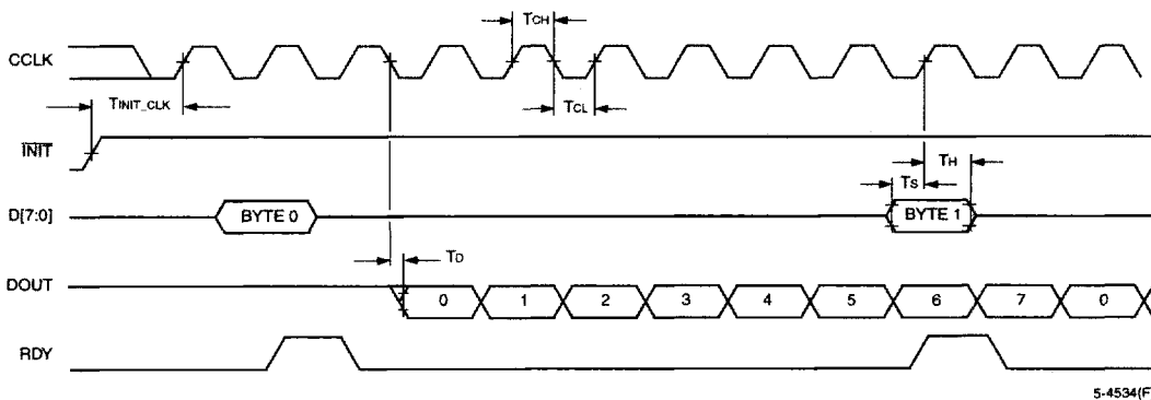
Figure 70. Synchronous Peripheral Configuration Mode Timing Diagram
