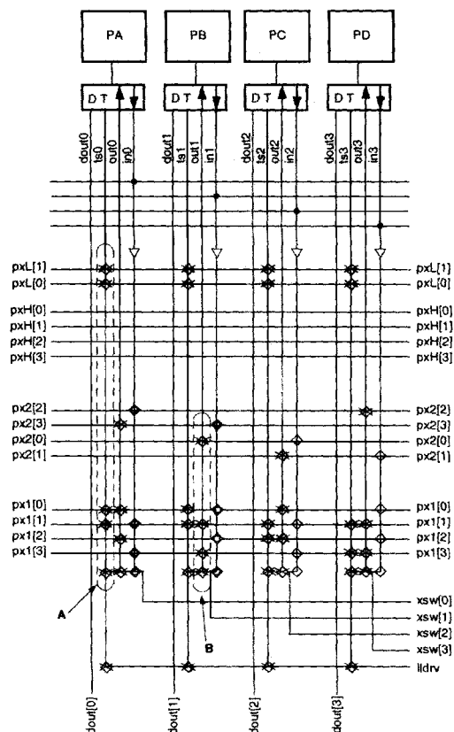
Figure 27. PIC Detail
