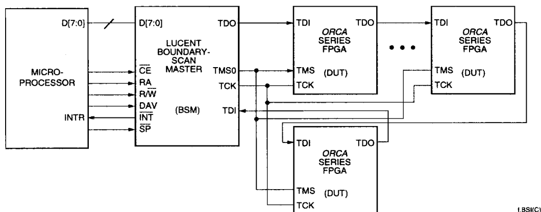
Figure 49. Boundary-Scan Interface
