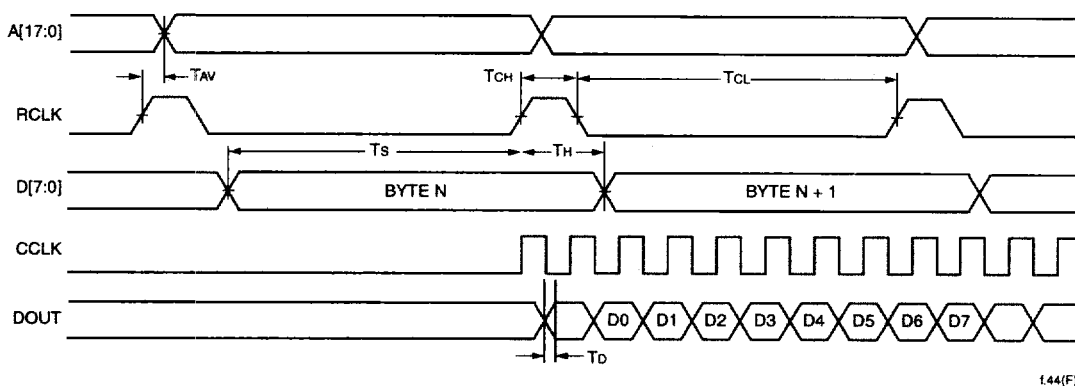
Figure 68. Master Parallel Configuration Mode Timing Diagram
