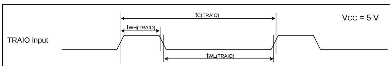
Figure 5.9 TRAIO Input Timing Diagram when V_{CC} = 5\text{ V}
