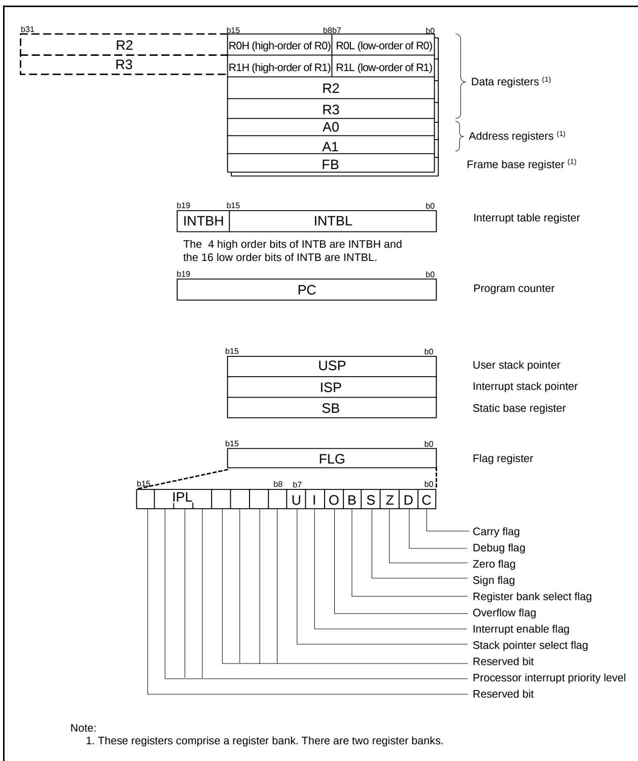
Figure 2.1 CPU Registers
