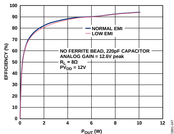
Figure 49. Efficiency vs. P_{OUT} , No Ferrite Bead, Analog Gain = 12.6 V peak, R_L = 8\ \Omega , PV_{DD} = 12\text{ V}
