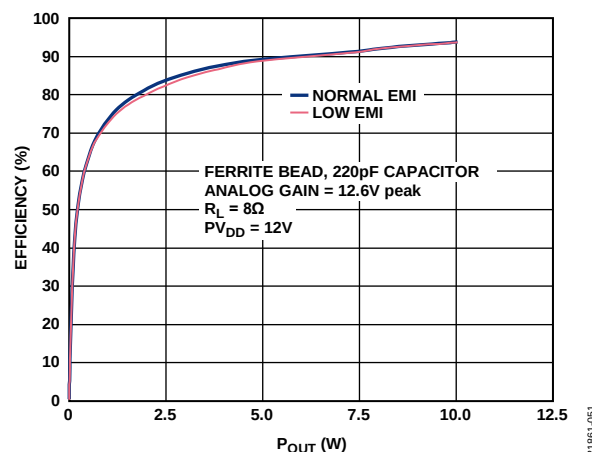
Figure 53. Efficiency vs. P_{OUT} , with Ferrite Bead, Analog Gain = 12.6 V peak, R_L = 8\ \Omega , PV_{DD} = 12\text{ V}
