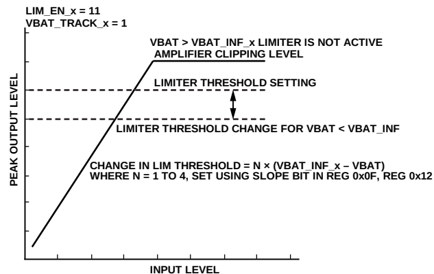
Figure 82. Limiter Example (LIM_EN_x = 11, VBAT_TRACK_x = 1)
