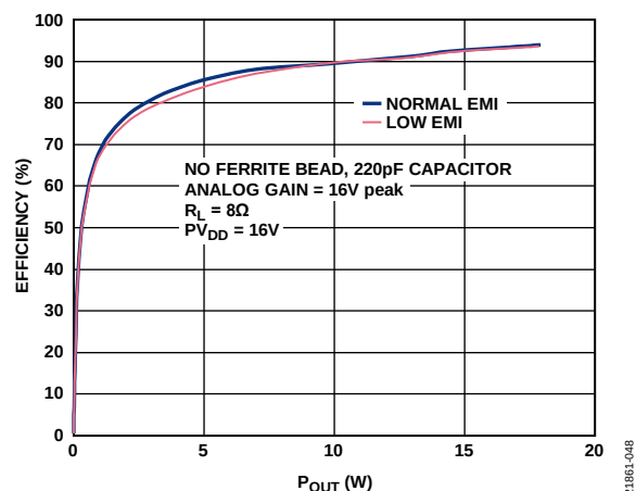
Figure 50. Efficiency vs. P_{OUT} , No Ferrite Bead, Analog Gain = 16 V peak, R_L = 8\ \Omega , PV_{DD} = 16\text{ V}
