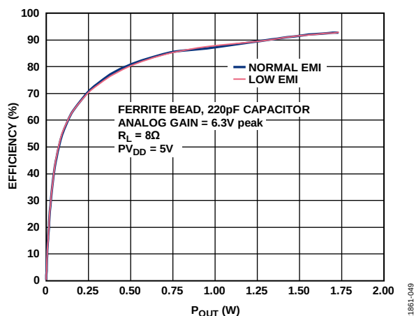
Figure 51. Efficiency vs. P_{OUT} , with Ferrite Bead, Analog Gain = 6.3 V peak, R_L = 8\ \Omega , PV_{DD} = 5\text{ V}
