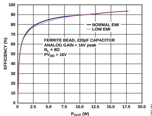
Figure 54. Efficiency vs. P_{OUT} , with Ferrite Bead, Analog Gain = 16 V peak, R_L = 8\ \Omega , PV_{DD} = 16\text{ V}
