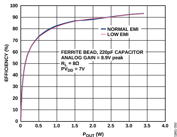
Figure 52. Efficiency vs. P_{OUT} , with Ferrite Bead, Analog Gain = 8.9 V peak, R_L = 8\ \Omega , PV_{DD} = 7\text{ V}
