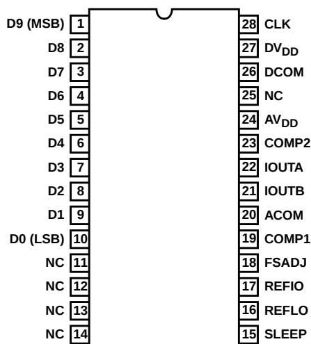
HI5760 (SOIC, SSOP) TOP VIEW
