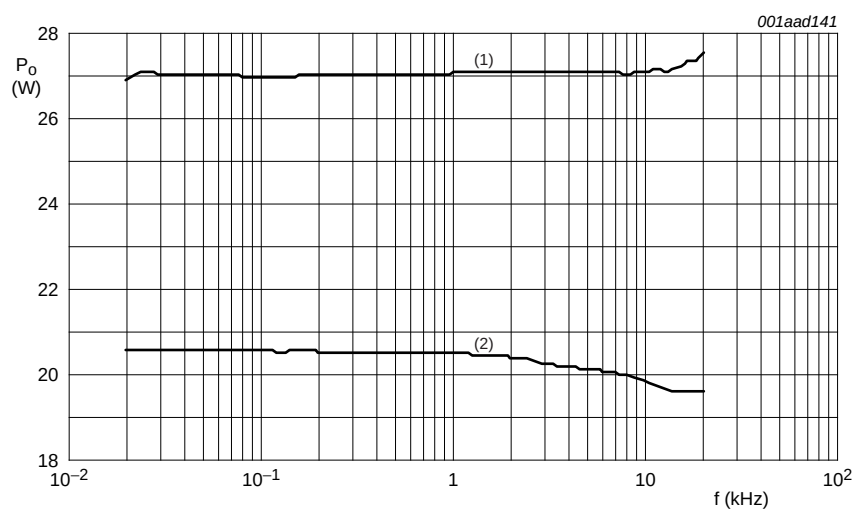
V_P = 14.4 V. (1) THD = 10 %. (2) THD = 0.5 %. Fig 20. Output power as a function of frequency; 4 \Omega load
