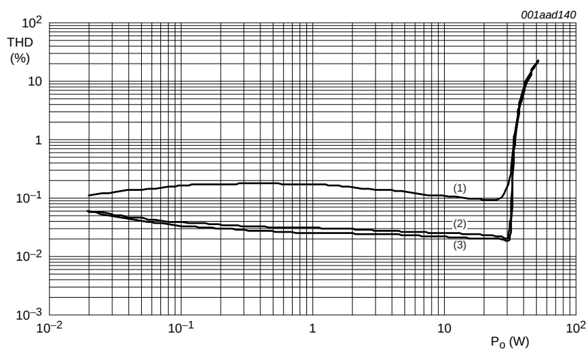
V_P = 14.4 V. (1) f = 10 kHz. (2) f = 100 Hz. (3) f = 1 kHz. Fig 19. Total harmonic distortion as a function of output power; 2 \Omega load
